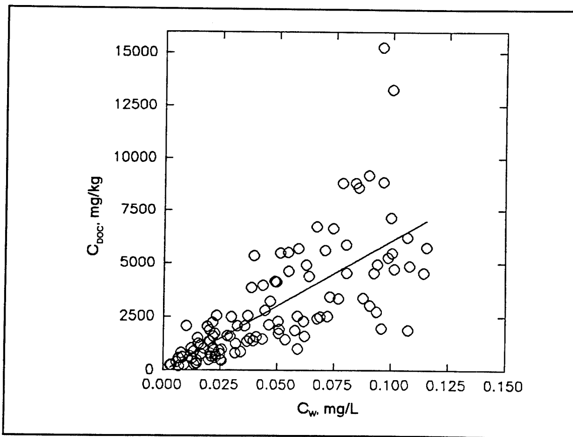
Figure 1. Truly dissolved ( C_w ) versus DOC normalized ( C_{\text{DOC}} ) fluoranthene concentrations in pore water
