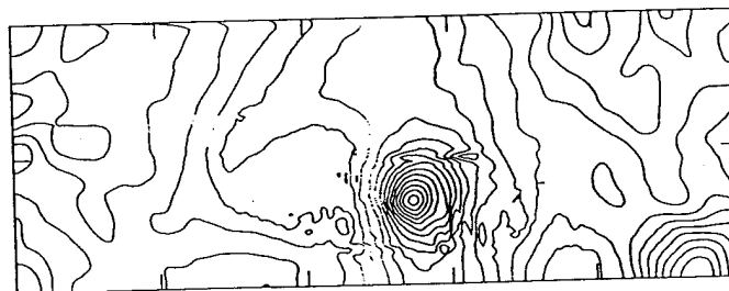
12. Computed Density, Vorticity, and Pressure Contours, M_s = 1.22 t = 1.09 ms
