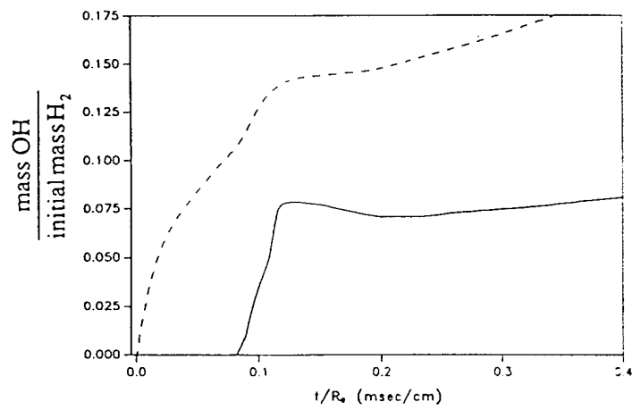
18. Consumption/Growth Histories of H_2 and OH , Initial Temperatures 1000^\circ K , 1500^\circ K
