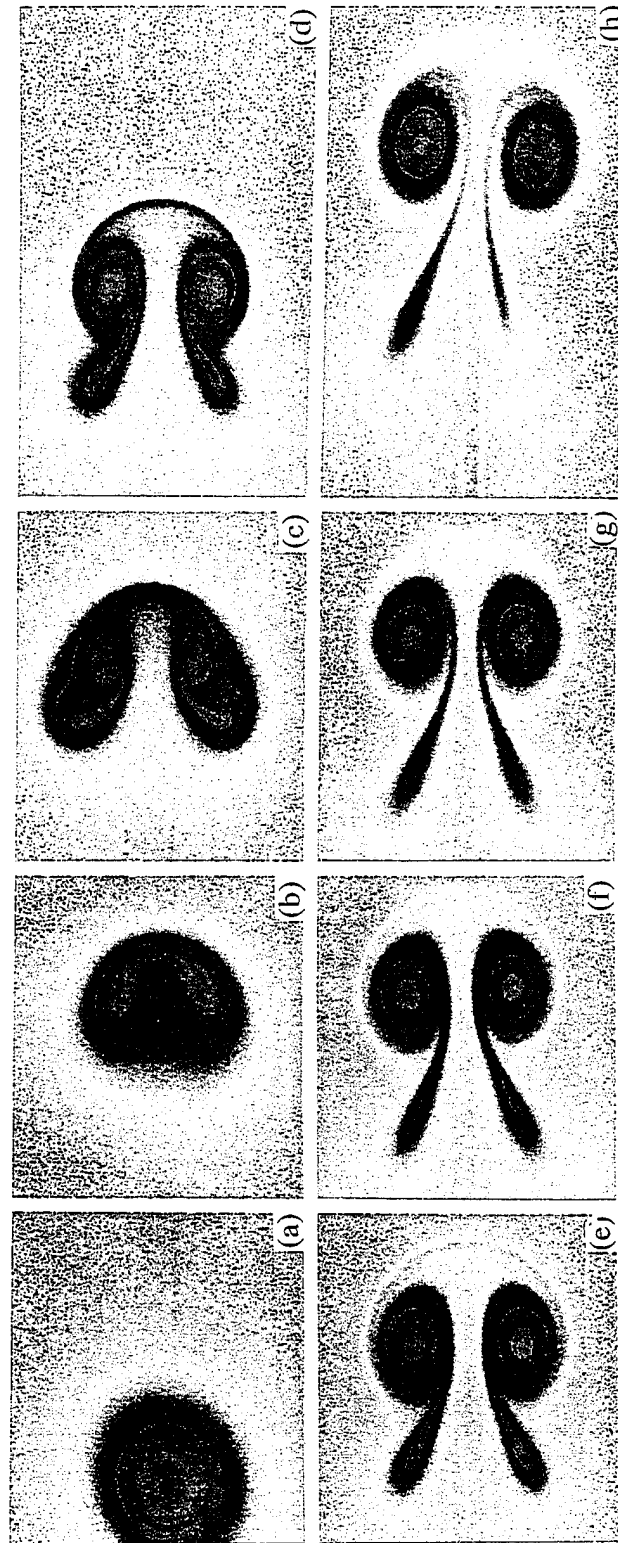
8. Rayleigh Scattering Images of Weak Shock Interaction with Helium Jet, M_S = 1.066 a) t = 0.0 ms b) t = 0.24 ms c) t = 0.70 ms d) t = 1.15 ms e) t = 1.72 ms f) t = 1.89 ms g) t = 2.13 ms h) t = 2.64 ms
