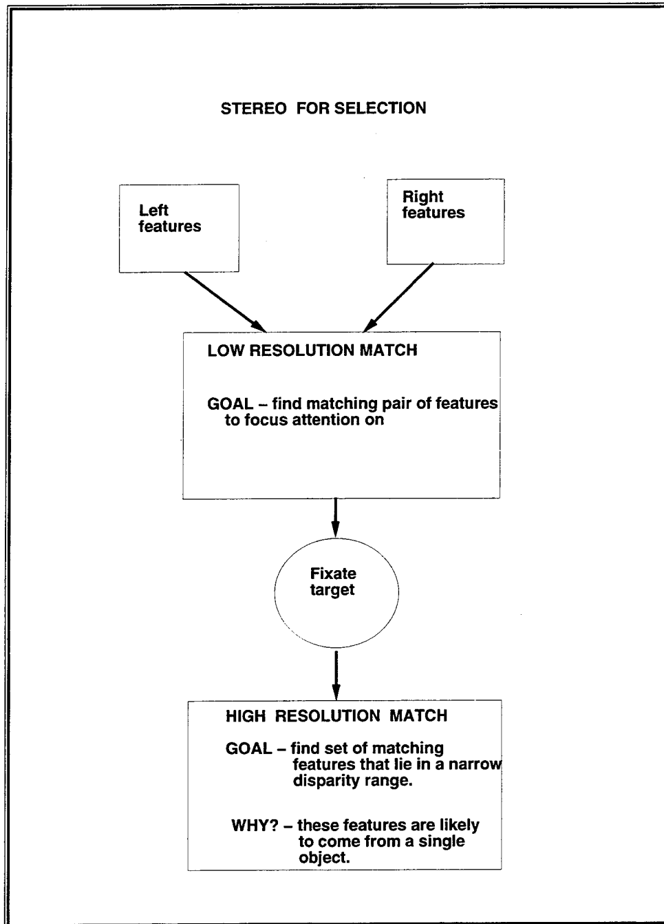
Figure 4-5: Stereo Algorithm.
