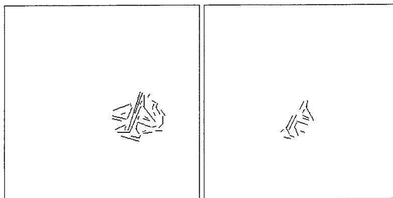
Figure 6-39: Segments from left and right images after applying color filter. Note that the color filter misses many segments on the object due to the change in the color of the light source.
