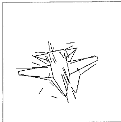
Figure 6-45: The model aligned with the selected segments. The verification system accepted this as a good alignment and gave us a false positive.
