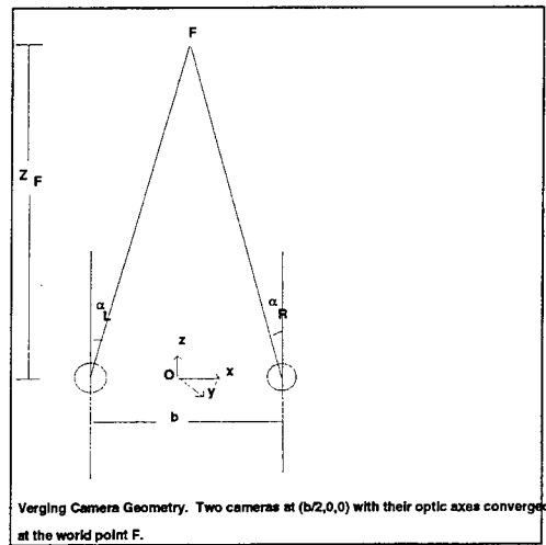
Figure 4-1: Camera geometry with baseline b , two cameras with focal length f verged such that each makes an angle of \alpha_l and \alpha_r with the line perpendicular to the baseline.
