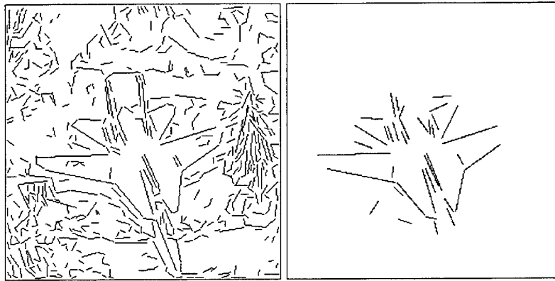
Figure 6-44: a) The segments in the image. b) The selected segments.
