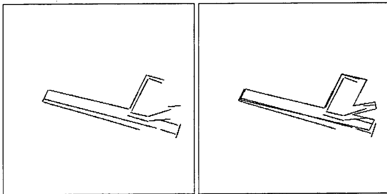
Figure 6-36: a) Selected segments b) Selected data aligned with model. As we can see, the alignment is good enough and the object is FOUND in the given scene.
