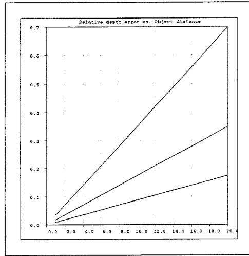
Figure 4-2: Plots of the percentage error in depth as a function of object distance (in units of interocular separation). Graphs represent errors in computing gaze angles of 1, 0.5 and 0.25 degrees, from top to bottom. This figure is taken from [24].
