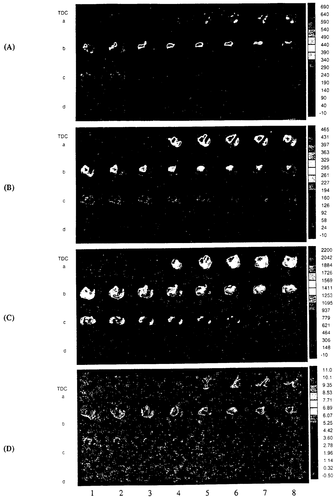
Fig. 6. Instantaneous IR Images Obtained in Exposure Period of 90\mu\text{sec} and Image Interval of 2.5\text{CA} from Engine Speed of 500\text{rpm} with Injection at 4\text{dTDC} . Images Obtained via Bands of (A) 2.2\text{-}2.5\mu\text{m} and (B) 4.5\text{-}5.5\mu\text{m} . Two-Color Method was Used to Calculate Distributions of (C) Temperature (K) and (D) KL Factor (in a relative scale).
