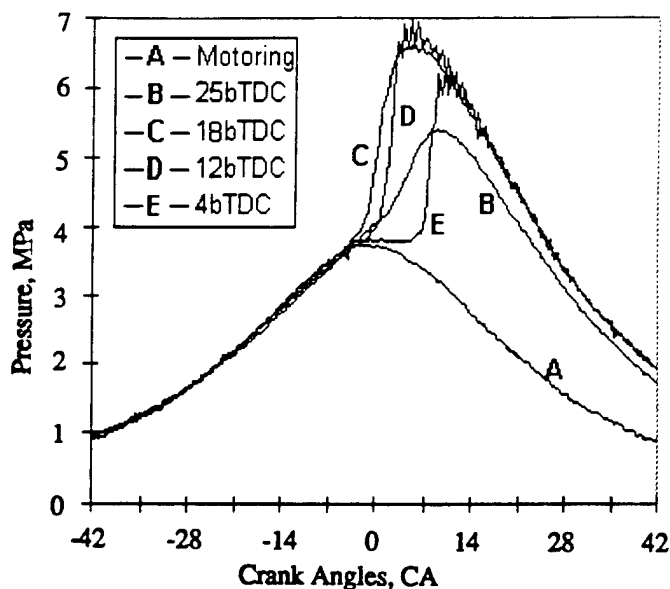
Fig. 5. Pressure-time Diagrams for Varied Injection Times and Hot-motoring Condition.
