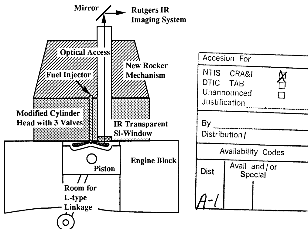
Fig. 1. Schematic Presentation of the Single Cylinder Engine Mounted by a Cummins 903 Cylinder Head with Optical Access for the SIS or Rutgers IR System.
