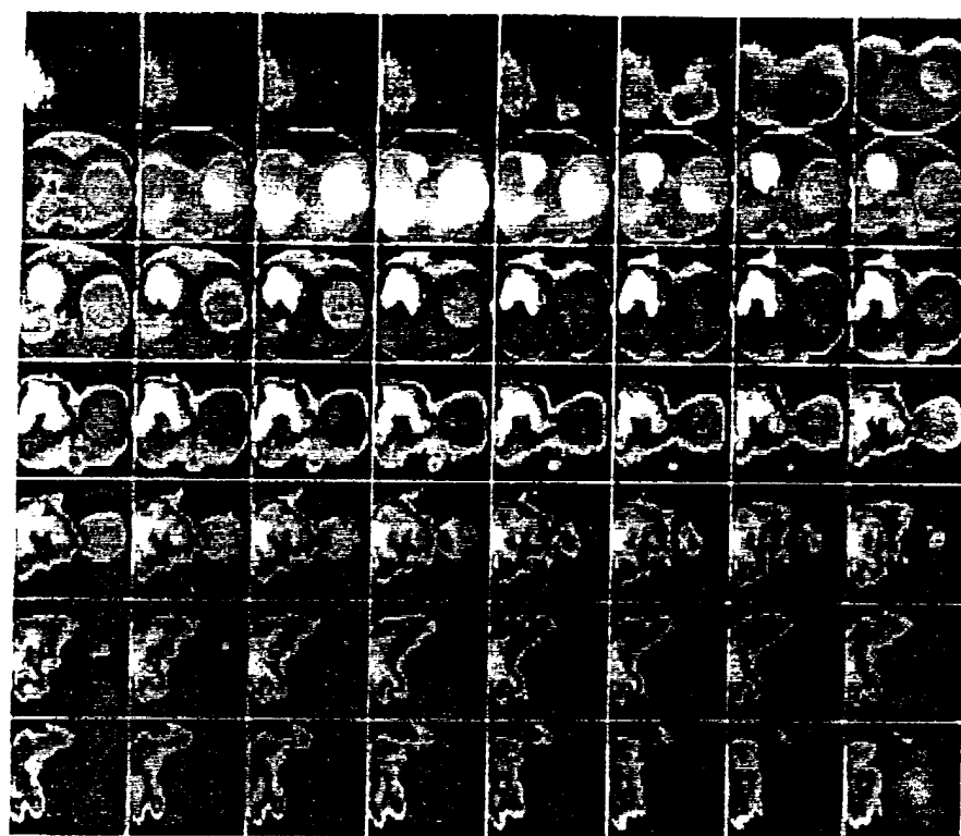
Fig. 7. High-speed Spectral IR Images of In-cylinder Events with a Gasoline-air Mixture near the Stoichiometric (Warm Engine): (A) 2.47\mu\text{m} and (B) 3.43\mu\text{m} .
