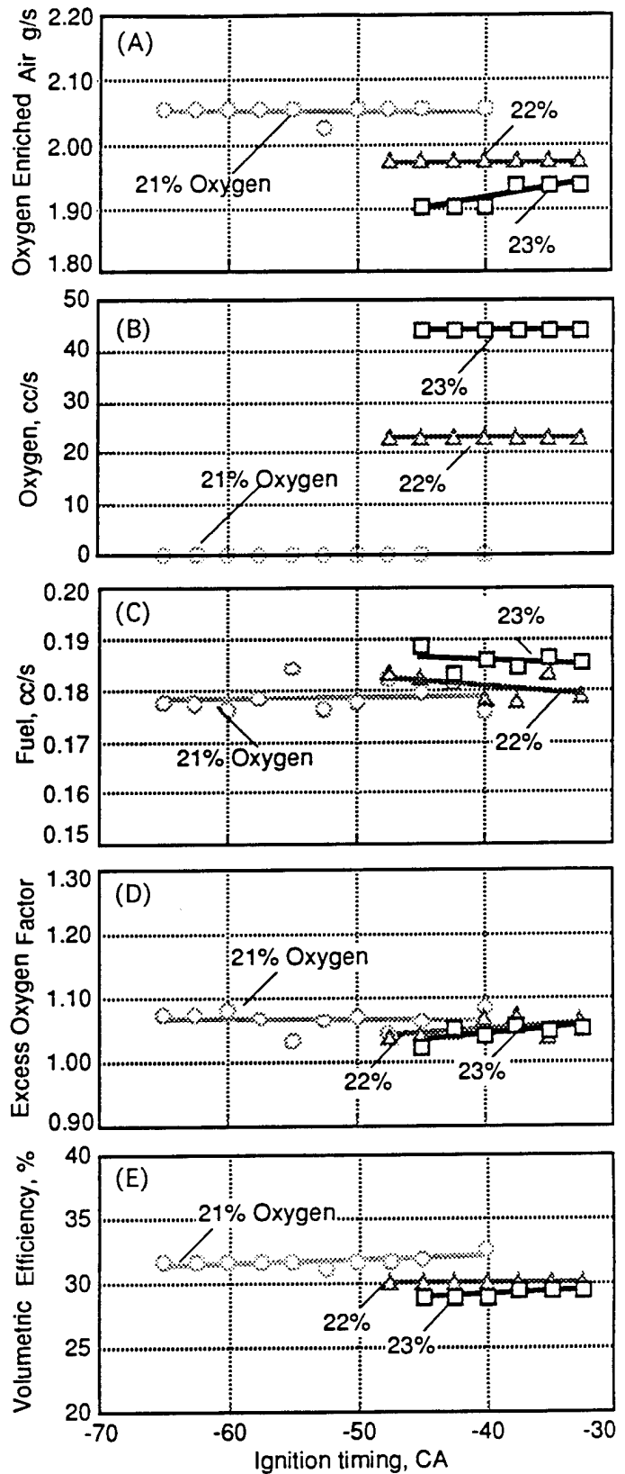
Fig. 3. Measurements Characterizing Engine Operation Conditions with the IOE.
