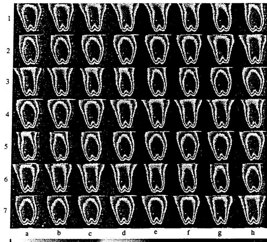
FIGURE 6 (A) High-Speed Spectral ( 2.2\text{--}2.5\ \mu\text{m} ) IR Images of Poiseuille-Flow Burner with 200 cc/sec Flow of 9% Natural Gas in Air Obtained at 200 frames/sec Having 90 \mu\text{sec} Exposure Period. See COLOR PLATE X.
