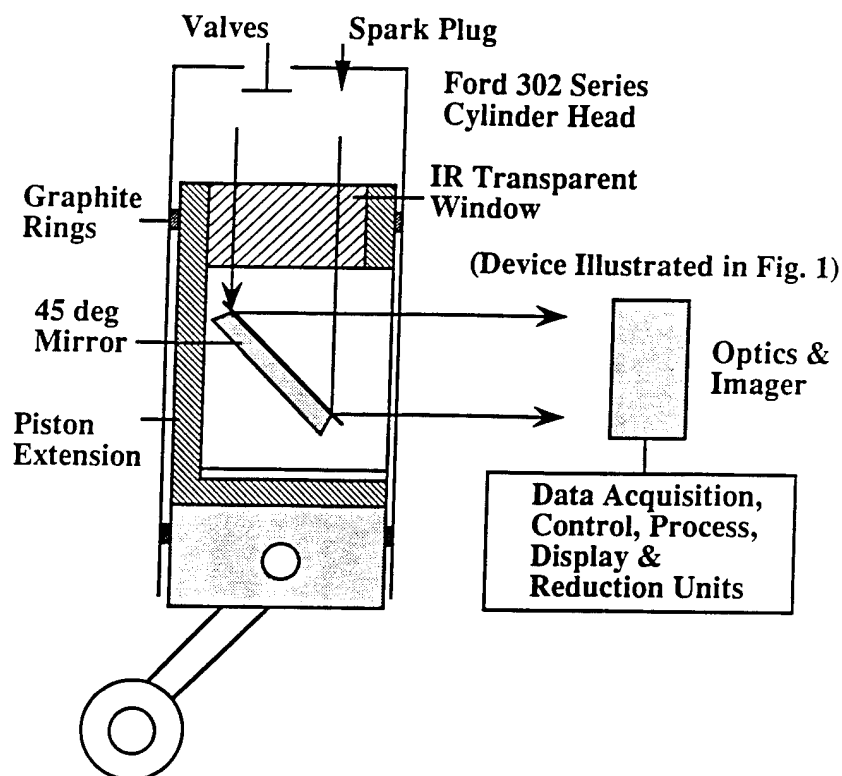
FIGURE 7. Schematics of SI Engine Apparatus Lined up with New Imaging system.
