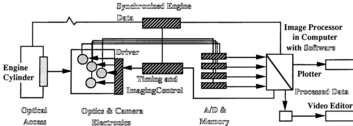
Fig. 4. (B) Optical Arrangement of the Rutgers Super Imaging System.
