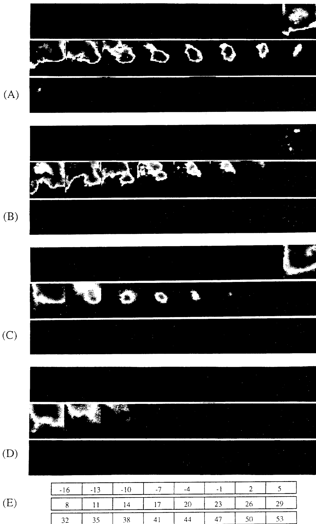
Fig. 9. High-Speed Spectral Infrared Images of In-Cylinder Reactions Obtained in (A) 2.47 \mu m, Neat Fuel; (B) 2.47 \mu m, MTBE-5; (C) 2.20 \mu m, Neat Fuel; (D) 2.20 \mu m, MTBE-5, and (E) Look-up Table.
