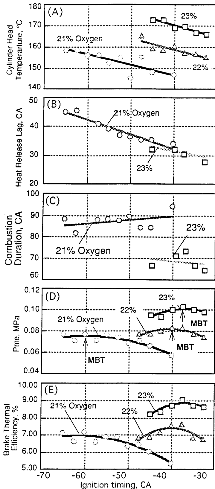
Fig. 4. Engine Performance and Condition Changes with the IOE.
