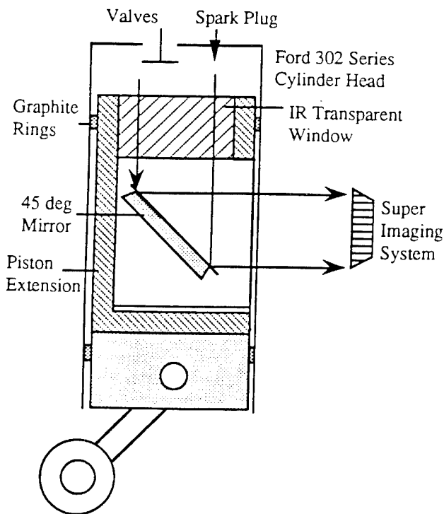
Fig. 4. The Spark-Ignition Engine with Optical Access.
