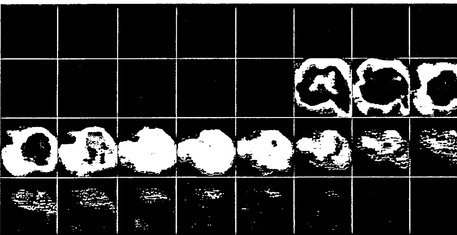
Fig. 6. High-speed Spectral IR Images of a Plume in CI-DI Engine Combustion Chamber in Band of 2.2-2.5 \mu m for Injection started at (1) 25bTDC; (2) 18bTDC; (3) 12bTDC and (4) 4bTDC.
