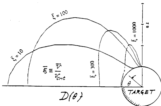
Fig. 3 Polar plot of local dimensionless deposition rate on a circular cylinder in crossflow for several values of the particle population size parameter \bar{v}/v_{crit} ; Cases shown: Threshold velocity for critical size particle rebound equal to ten times the mainstream velocity, U (after [R9]). Note tendency to form off-axis 'lobes' when \bar{v}/v_{crit} exceeds about 100.
