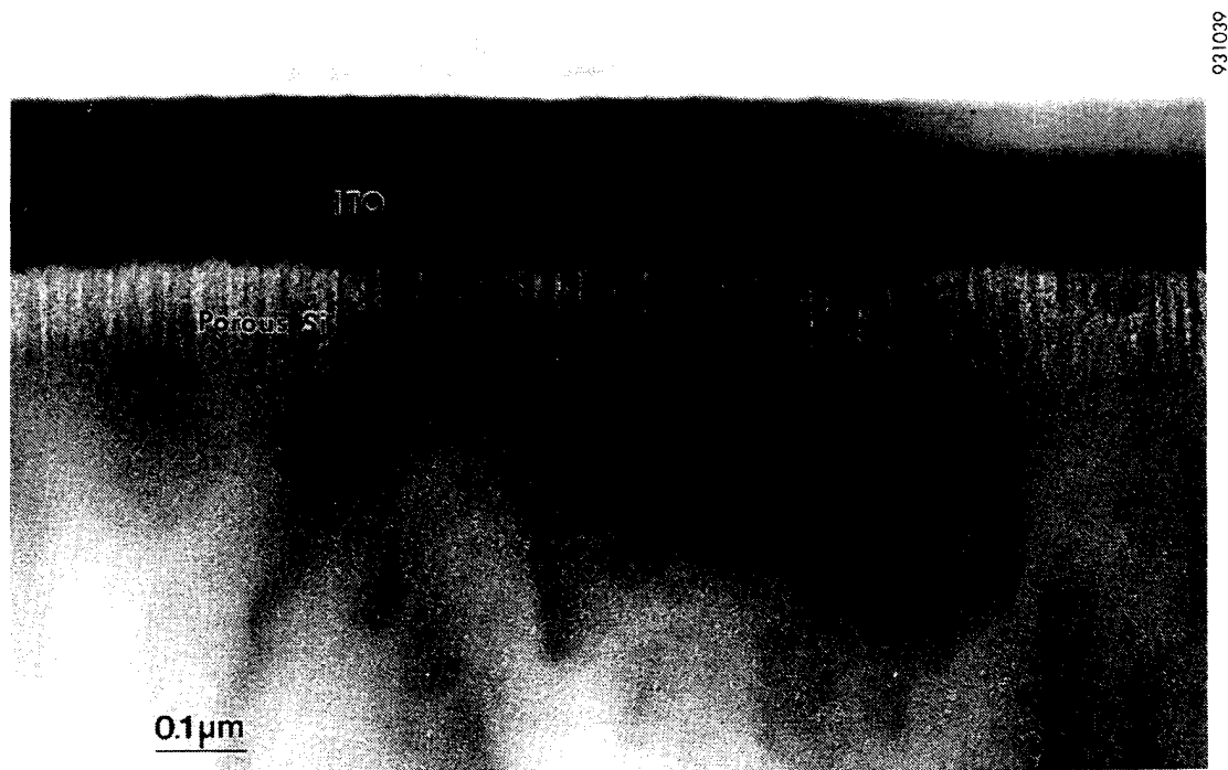
Figure 16 Cross-sectional view of a porous Si LED determined by TEM.
