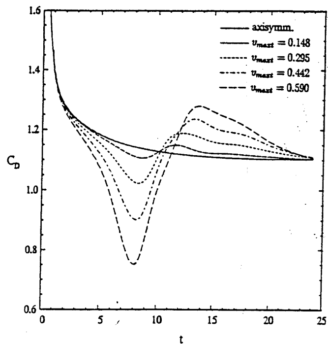
Figure 5. Drag coefficients of the sphere under the same conditions of figure 3.
