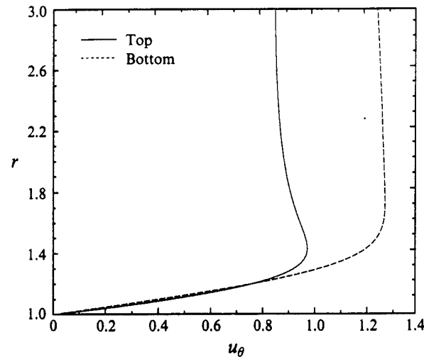
FIGURE 7. Tangential velocity profile, u_\theta(r) , at \theta = 90^\circ on the top and the bottom of the sphere in the principal plane at t = 12 .
