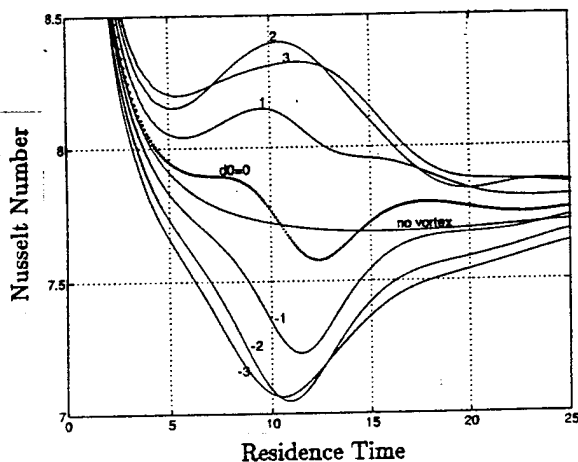
Fig. 4. Variation of the droplet Nusselt number versus the vortex initial offset distance. (This result is for v_{max} = 0.4 , Re = 100 , and \sigma = 1 .)
