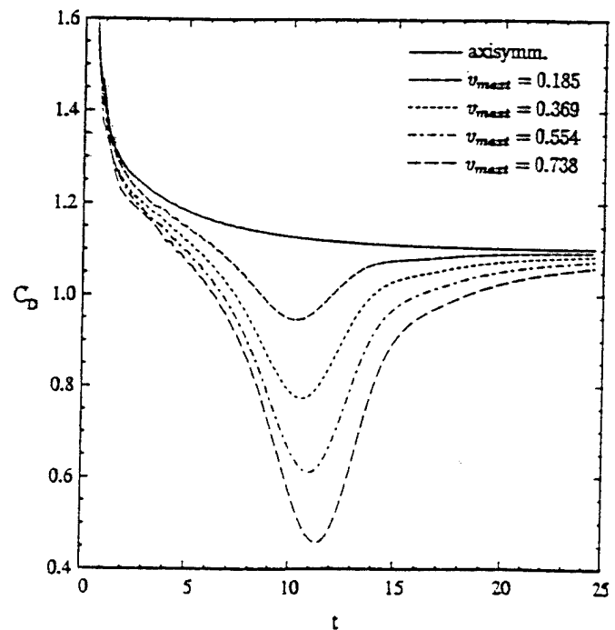
Figure 10. Drag coefficients of the sphere as a function of time and v_{max} for Re = 100 , d_{off} = \pm 1.5 , and \sigma = 1 with top-negative and bottom-positive circulations.
