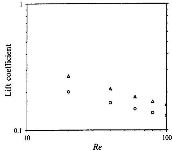
FIGURE 19. Root mean square of the lift coefficient and maximum positive lift coefficient as a function of Reynolds number under the same conditions as figure 17. \Delta , max; \circ , r.m.s.
