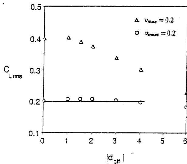
Figure 6. Rms lift coefficients of the sphere as a function of |d_{off}| for Re = 100 and \sigma = 4 .
