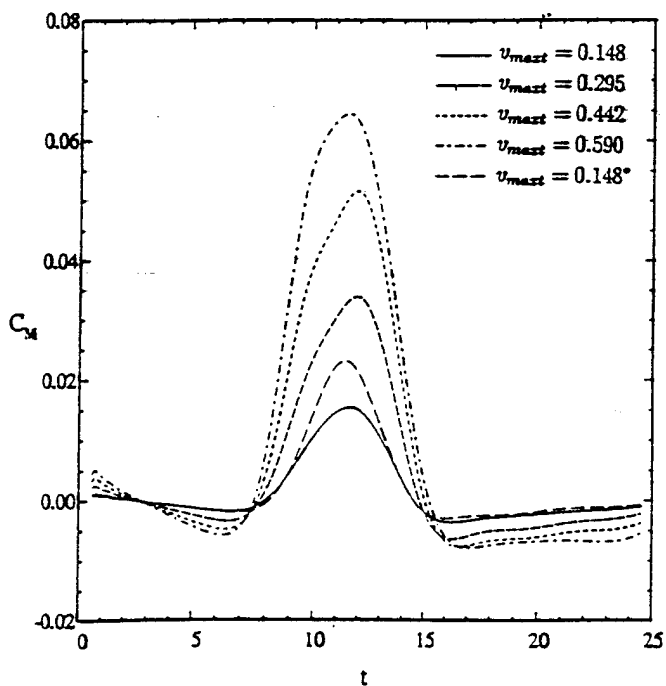
Figure 4. Moment coefficients of the sphere under the same conditions of figure 3. * denotes the case of a single vortex.
