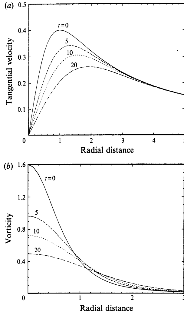
FIGURE 3. (a) Velocity and (b) vorticity fields due to a vortex tube as a function of radial distance and time for Re = 100 , \Gamma_v = 2.5 and \sigma = 1 .
