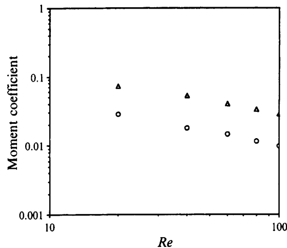
FIGURE 20. Maximum moment coefficient and root mean square of the moment coefficient as a function of Reynolds number under the same conditions as figure 17. \Delta , max; \circ , r.m.s.
