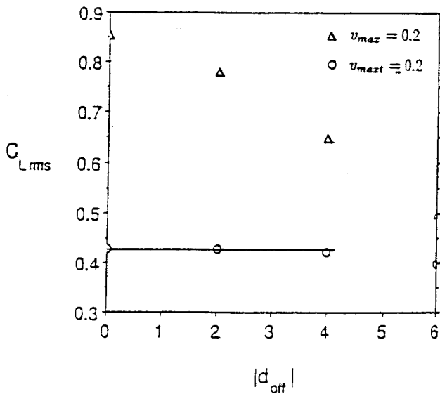
Figure 8. Rms lift coefficients of the sphere as a function of |d_{off}| for Re = 20 and \sigma = 4 .
