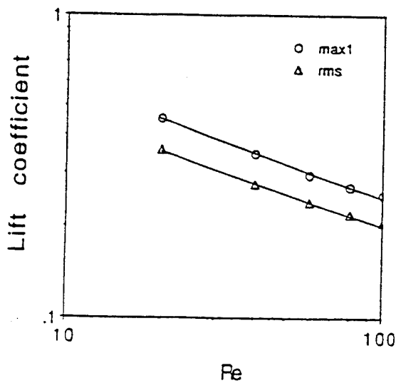
Figure 7. Maximum positive lift coefficient and rms lift coefficient as a function of Reynolds number for d_{off} = \pm 1.5 and \sigma = 1 with v_{max} = 0.295 .
