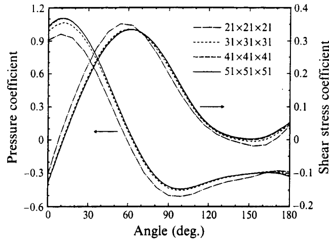
FIGURE 4. Pressure and shear stress distributions around the sphere in the (x, z) -plane of symmetry as a function of grid resolution at t = 12 for Re = 100 , d_{off} = 0 , \sigma = 1 , and v_{max} = 0.4 .
