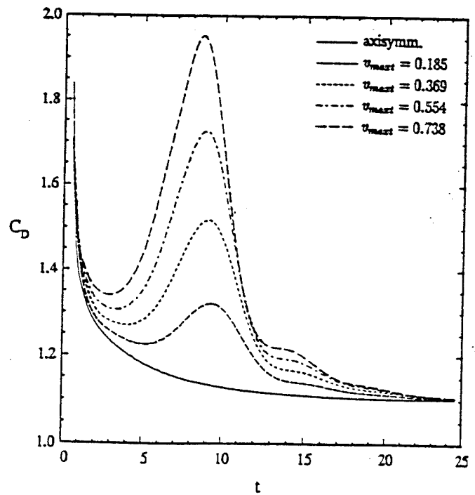
Figure 9. Drag coefficients of the sphere as a function of time and v_{max} for Re = 100 , d_{off} = \pm 1.5 , and \sigma = 1 with top-positive and bottom-negative circulations.
