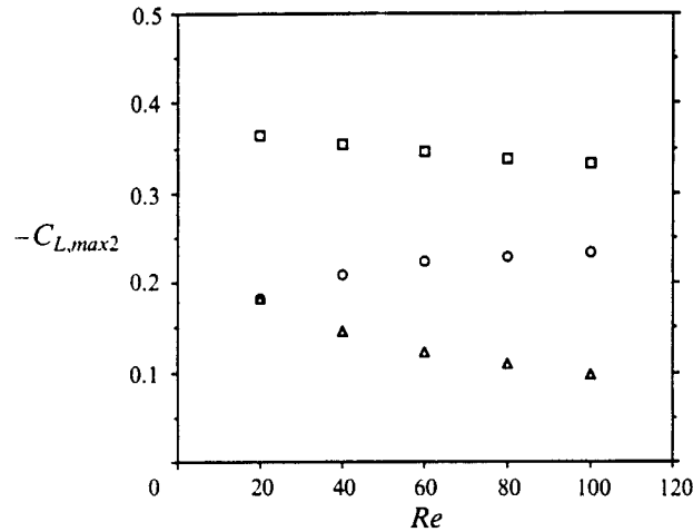
FIGURE 18. Total maximum negative lift coefficient and the coefficients due to pressure and viscous contributions as a function of Reynolds number under the same conditions as figure 17. \square , total; \circ , pressure; \triangle , viscous.
