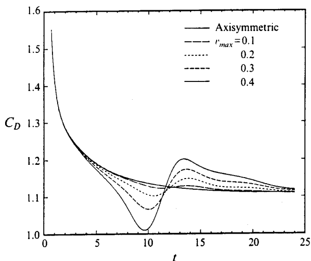
FIGURE 11. Drag coefficients of the sphere under the same conditions as figure 9.
