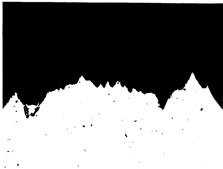
Figure 1.8: Digitization of crack profile of which dimensions are actual.
