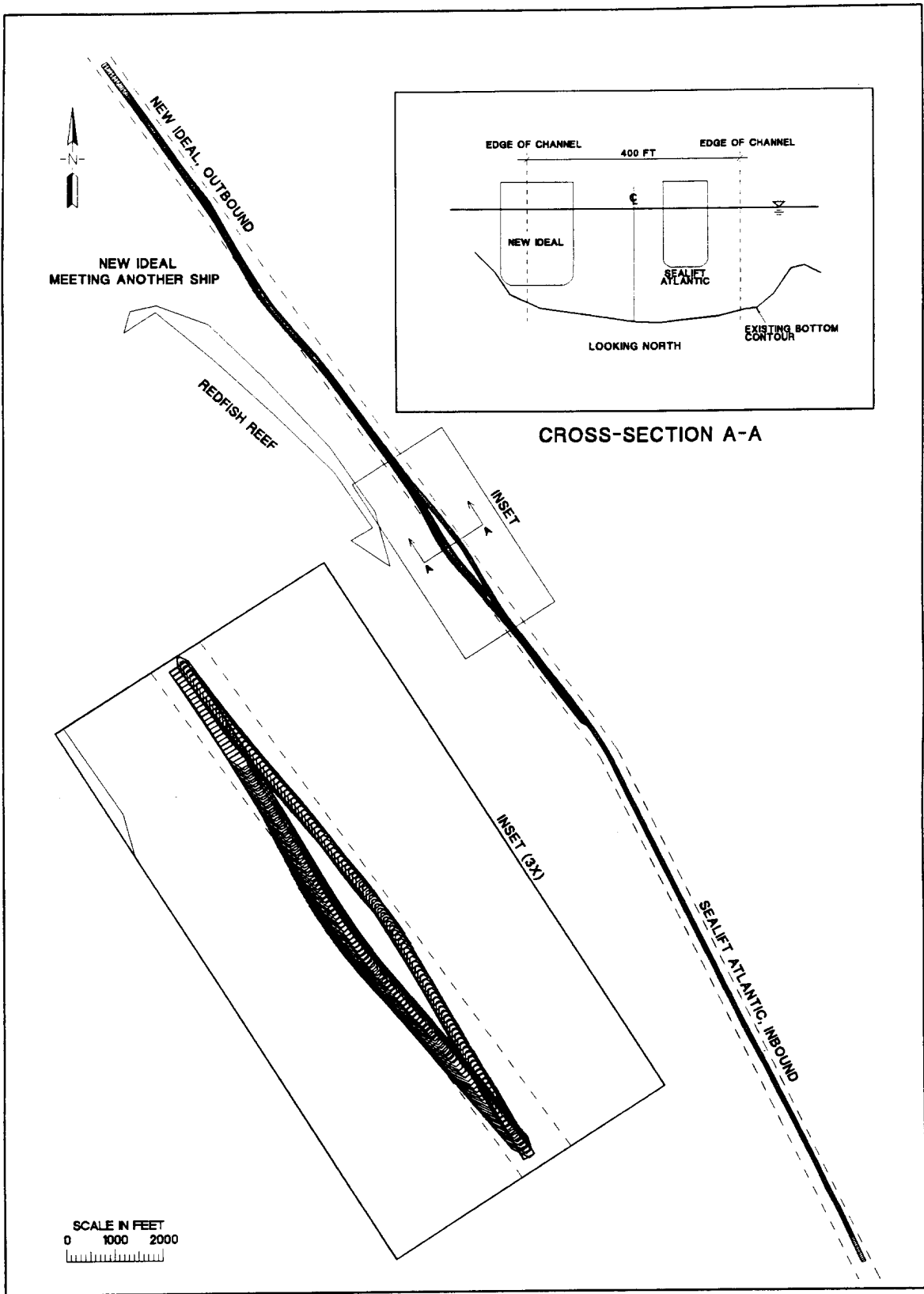
Figure 18. Track plot of DGPS vessels
