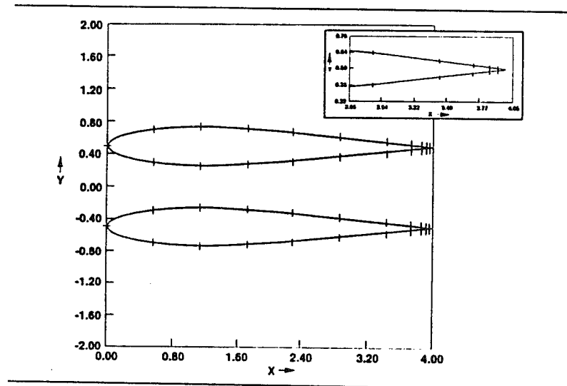
Figure 14 Sample discretization for problems A.5 and A.7.
