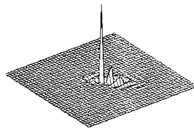
Inverse PSF - Wiener
