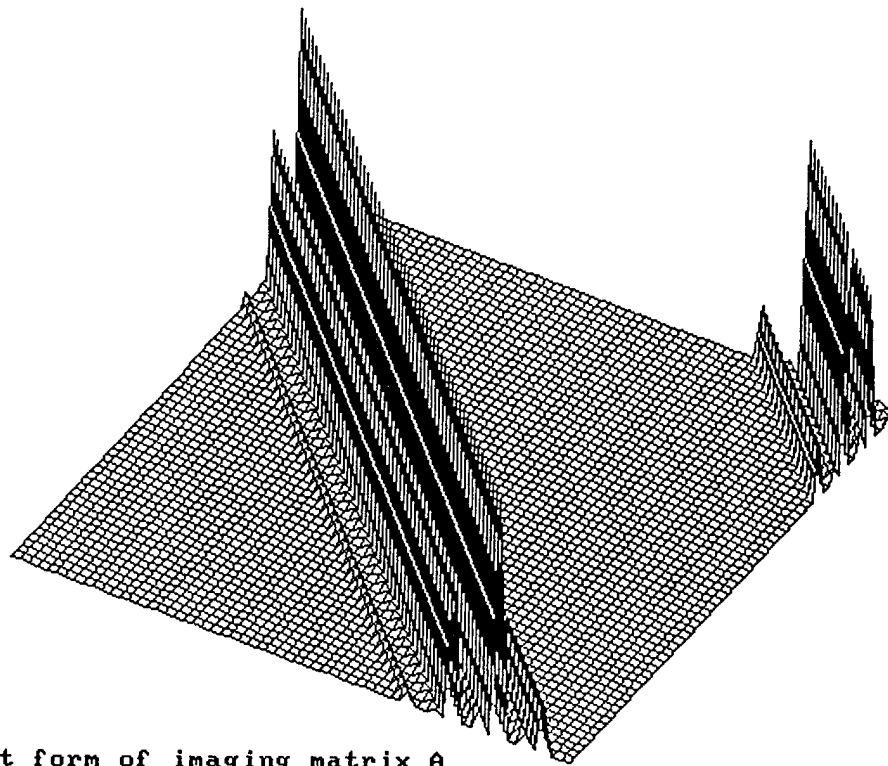
circulant form of imaging matrix A 625x625 elements
