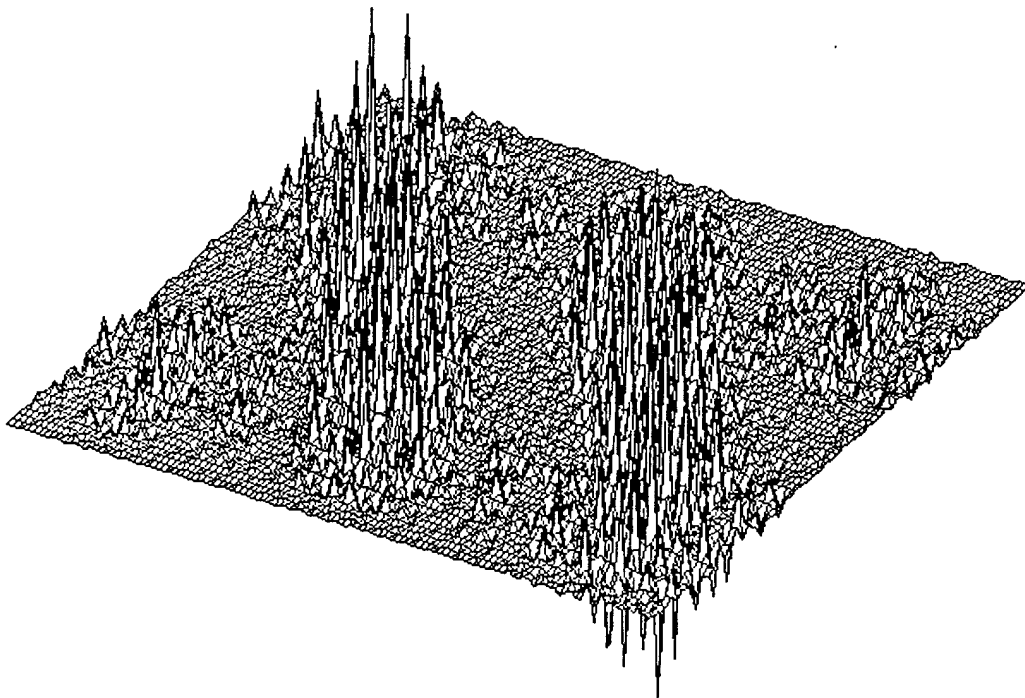
deconvolution matrix obtained from svd of A
