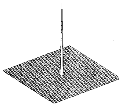
Processed PSF - Wiener
