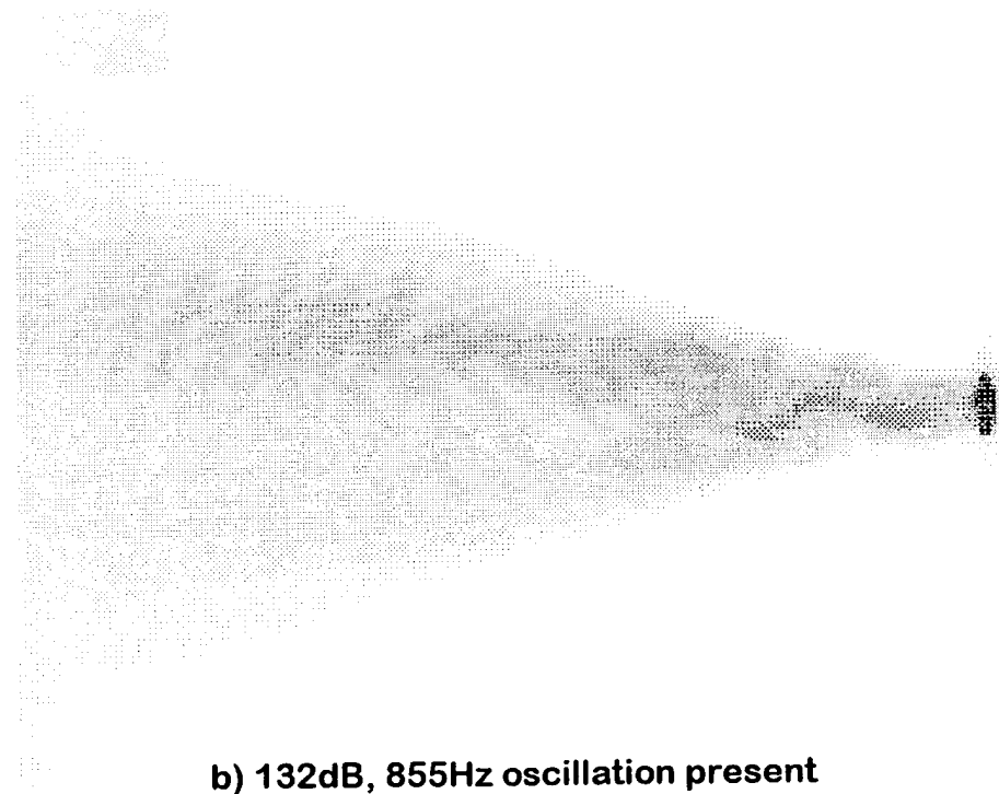
Figure 14. Phase-locked, averaged images of a jet excited by transverse acoustic oscillations.
