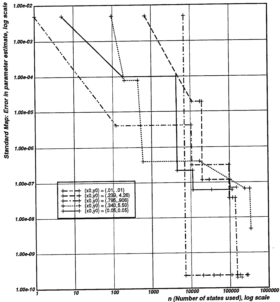
Figure 6.14: This graph depicts the performance of the proposed algorithm for estimating parameter K using one sequence of noisy state data from the standard map with K = 1 .
