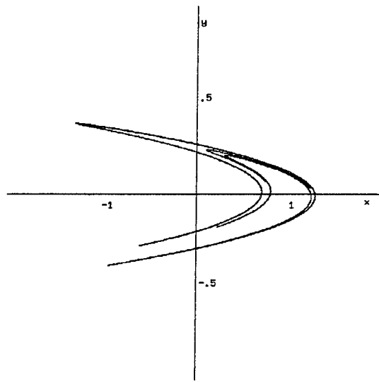
Figure 6.7: The Henon attractor for a = 1.4 , b = 0.3 .
