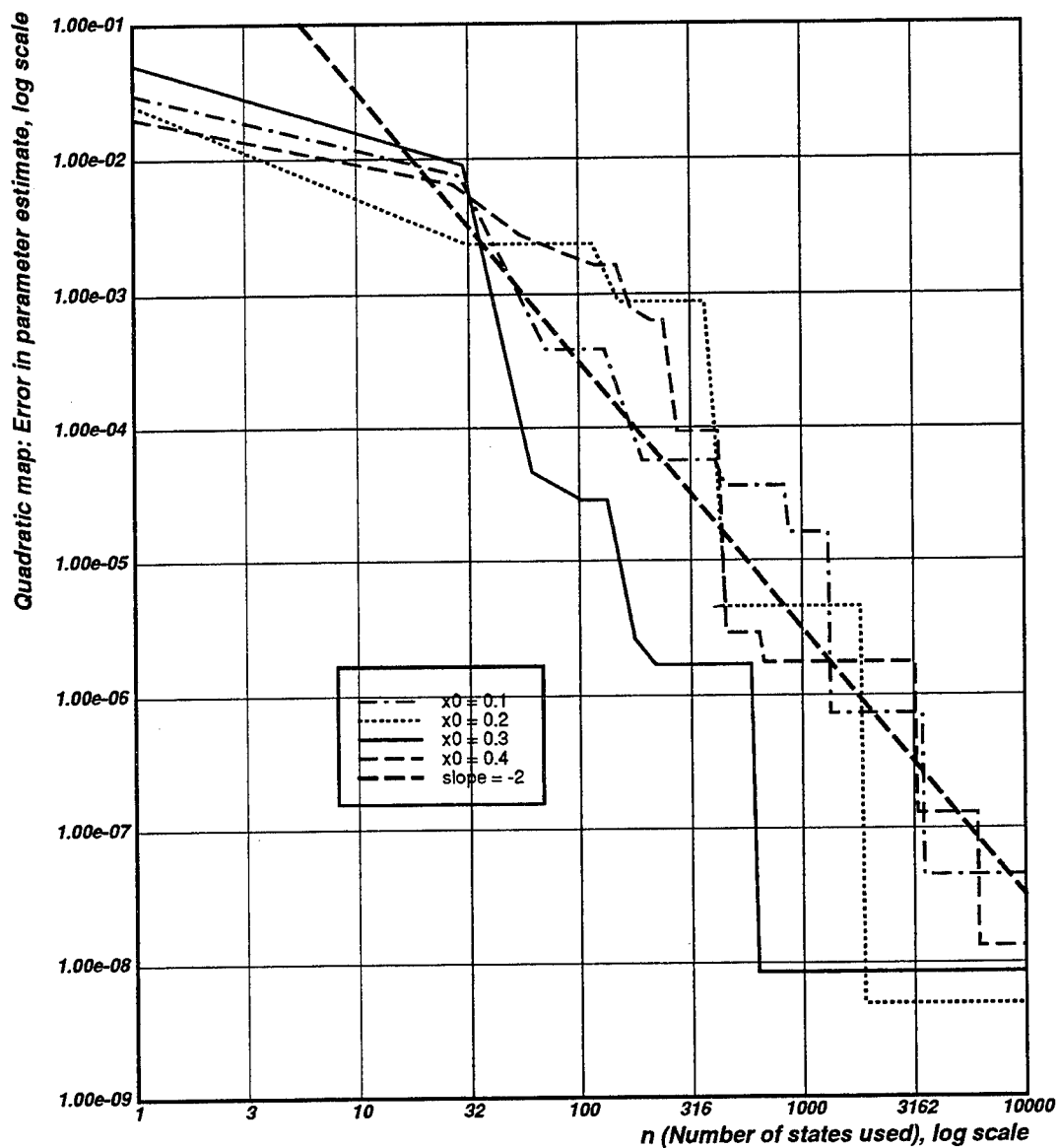
Figure 6.5: Graph of the actual error in the parameter estimate of the proposed algorithm when applied to data from the quadratic map with p = 3.9 . A line of slope -2 is drawn on the graph to indicate the conjectured asymptotic rate of convergence for the estimate.
