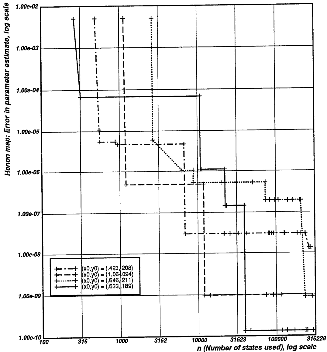
Figure 6.10: Graph of the actual error of the parameter estimate for a using the proposed algorithm on the Henon map (with a = 1.4 and b = 0.3 ). This graph contains results for four different sets of data corresponding to four different initial conditions, all chosen on the attractor of the system. The tick marks on each trace denote places where the top level Kalman filter deferred to a Monte-Carlo-based approach for additional analysis.
