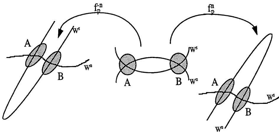
Figure 5.4: Here we illustrate why there can be multiple regions shadowing the same orbit. Near areas of folding, two regions, A and B , can be separate, yet can get asymptotically mapped toward each other both forwards and backwards in time. Note that in the picture, A and B are located at intersections of the same stable and unstable manifolds. This situation must be dealt with when sampling probability densities and searching for optimal shadowing orbits.
