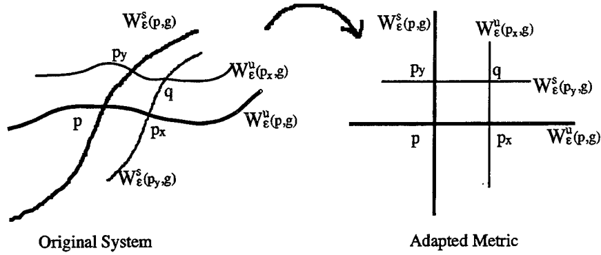
Figure 2.1: First we use the structure of the manifolds of the hyperbolic system to define a local coordinate system with nice geometric properties, so that the manifolds are orthogonal and and expand/contract uniformly under a single application of g .
