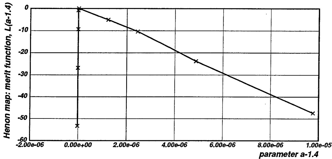
Figure 6.9: Asymmetry in the parameter space of the Henon map (with a = 1.4 , b = 0.3 ): Here we graph the parameter merit function L(a) after 200000 iterates of an orbit with initial condition on the attractor near x_0 = (.423, .208) . Note that this merit function is actually based on only the most sensitive 931 data points, since the linear filter threw out over 199,000 points.
