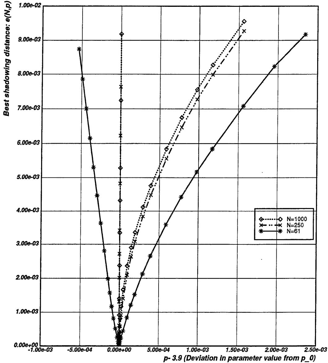
Figure 1.1: Graph of best shadowing distance, e(N, p) , with respect to p , for f_p = px(1 - x) , p_0 = 3.9 and x_0 = 0.3 . e(N, p) measures how closely an orbit of f_p can shadow a fixed orbit, \{x_n\}_{n=0}^N , of f_{p_0} . On the x -axis of the graph, p is labeled as p - p_0 , the difference in parameter value from the parameter used to generate \{x_n\}_{n=0}^N . e(N, p) is plotted on the y -axis with N held constant for three different values of N . The three v-shaped curves represent e(N, p) for N = 61 , N = 250 , and N = 1000 . Note the distinct asymmetry in how well orbits of f_p track \{x_n\}_{n=0}^N for p > p_0 and p < p_0 .
