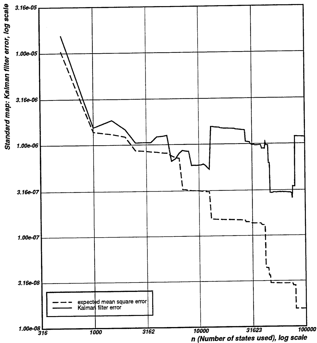
Figure 6.12: This graph depicts the performance of the square root extended Kalman filter for estimating parameter K using one sequence of noisy state data from the standard map with K = 1 . The data was generated using the initial condition, (x_0, y_0) = (0.05, 0.05) . This initial condition results in a trajectory that wanders around in a chaotic zone.
