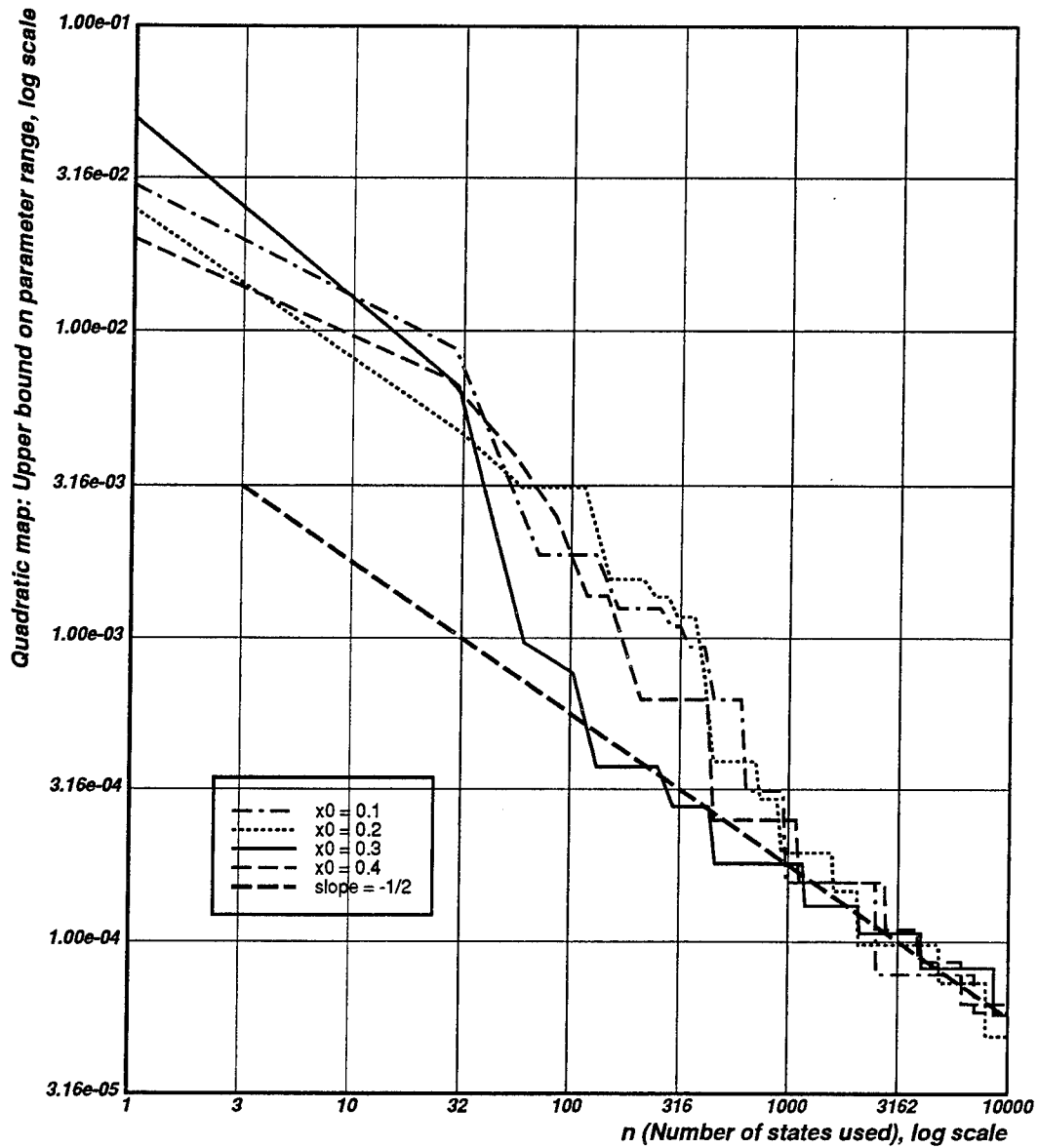
Figure 6.6: Graph of the error in the upper bound of the parameter range being considered by the proposed algorithm for the quadratic map with p = 3.9 . A line with a slope of -\frac{1}{2} is drawn to indicate the expected asymptotic convergence of the error.
