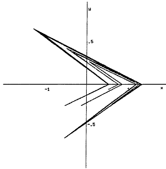
Figure 6.15: The Lozi attractor for a = 1.7 , b = 0.5 .
