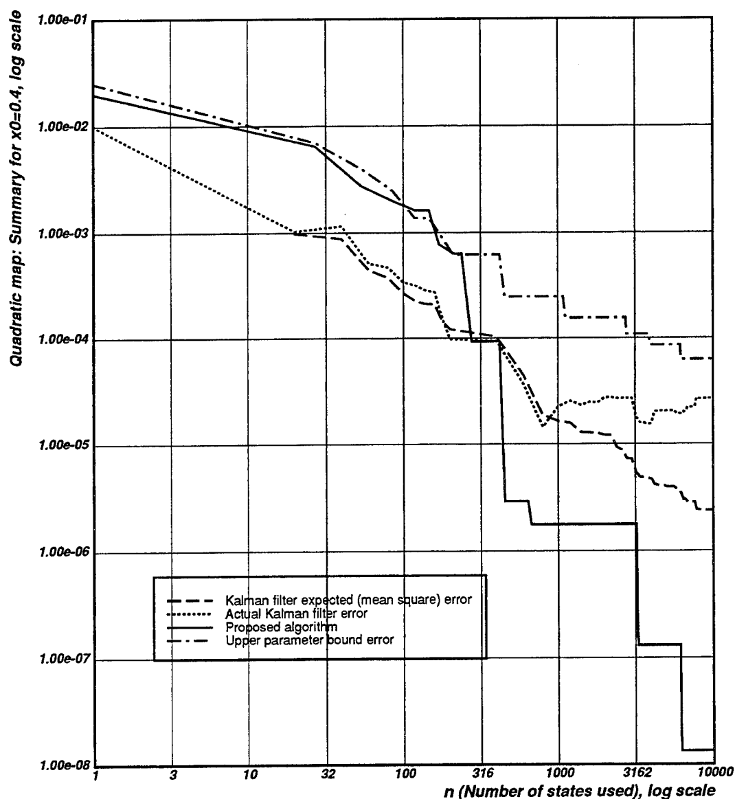
Figure 6.1: This graph summarizes results related to estimating the parameter p in the quadratic map for data generated using the initial condition x_0 = 0.4 .
