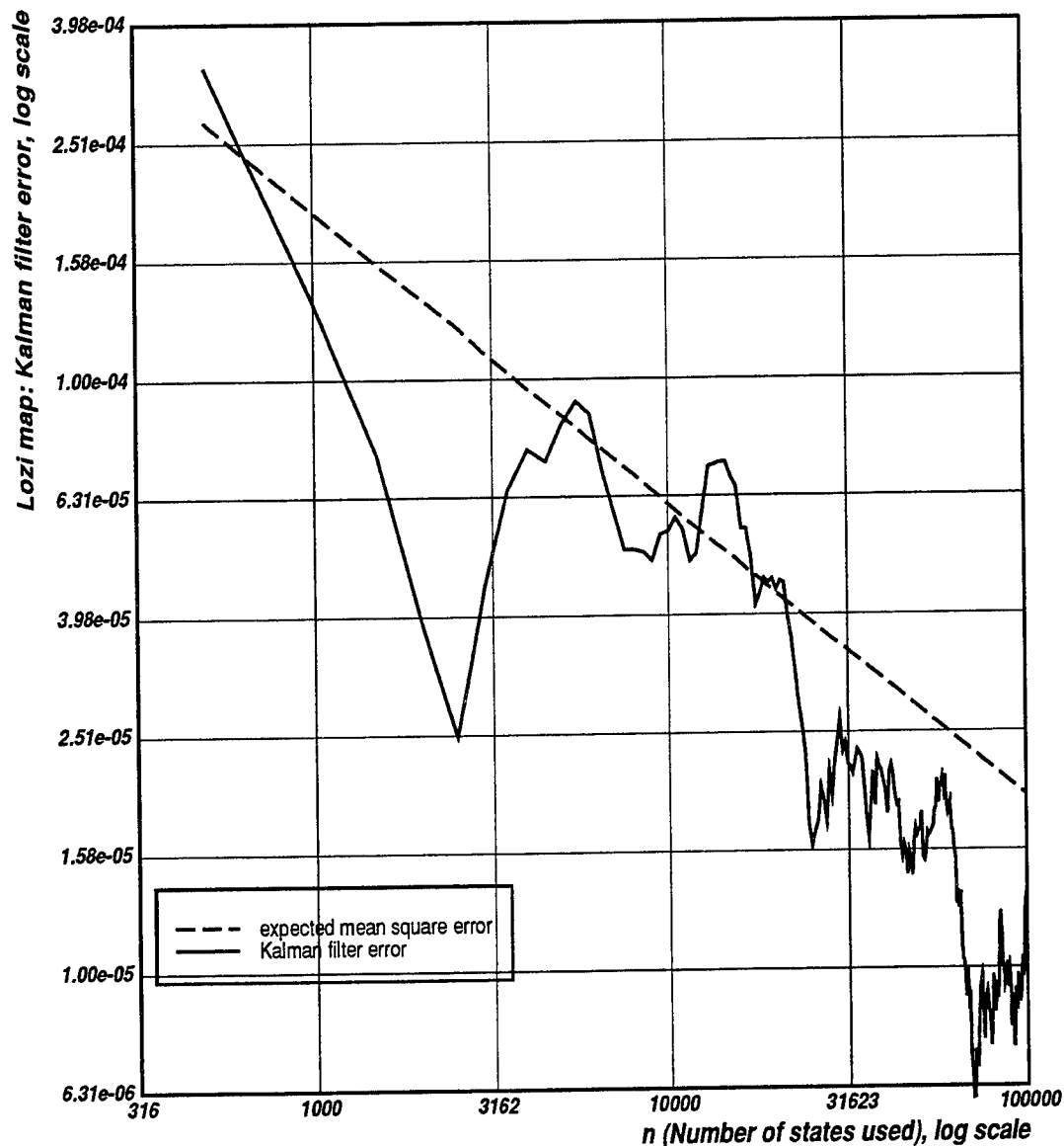
Figure 6.16: This graph plots the performance of a square root extended Kalman filter in estimating the parameter, a , in the uniformly hyperbolic Lozi map. The data here represents the average over five runs based on data with different measurement noises bit generated using the parameters a = 1.7 , b = 0.5 , and the same initial condition on the attractor, near (x_0, y_0) = (-.407, .430) . Note the lack of divergence, and the fact that convergence is purely stochastic.
