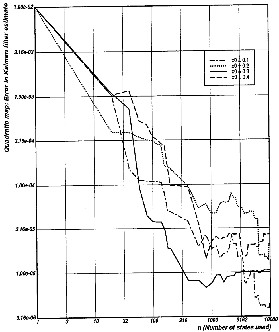
Figure 6.3: Graph of the average error in the parameter estimate as computed by square root extended Kalman filter applied to the quadratic map with parameter value p = 3.9 . Data represents average error over 10 runs.
