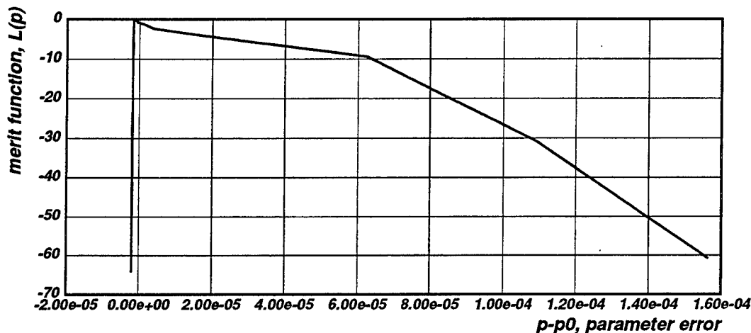
Figure 6.4: Asymmetry in the parameter space of the quadratic map: Here we graph the parameter merit function L(p) after processing 2500 iterates of an orbit with initial condition x_0 = 0.4 . The merit function is normalized so that L(p) = 0 at the maximum. Since \sigma = 8 , a parameter sample, p , is deleted if L(p) < -64 . This sort of asymmetrical merit function is typical of all orbits encountered in the quadratic map, Henon map, and standard map.
