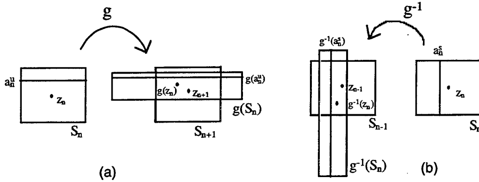
Figure 2.2: For any \epsilon > 0 we can choose \delta > 0 so that for any n \in \mathbb{Z} , (a) any line segment, a_n^u , along the unstable direction in S_n gets mapped by g so that it intersects S_{n+1} , and (b) any line segment, a_n^s , along the stable direction in S_n gets mapped by g^{-1} so that it intersects S_{n-1} .
