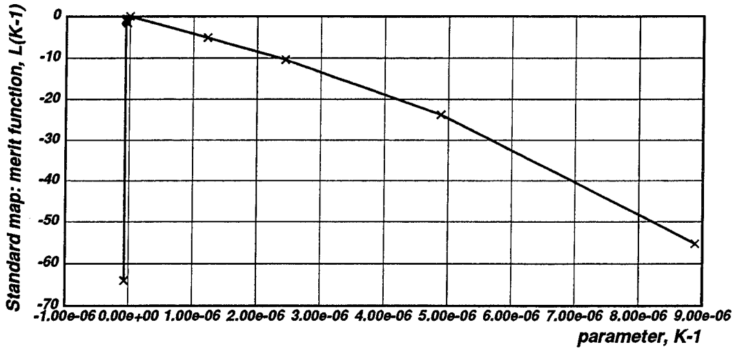
Figure 6.13: Asymmetry in the parameter space of the standard map (with K = 1 ): Here we graph the parameter merit function L(K) after 250000 iterates of an orbit with initial condition x_0 = (.423, .208) .
