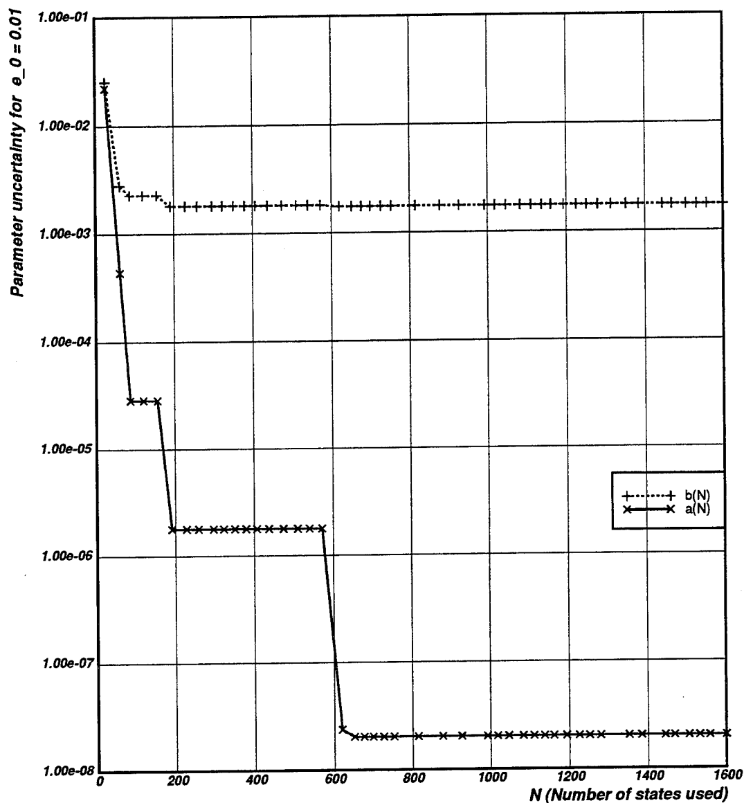
Figure 1.2: Graph of a(N) and b(N) with respect to N for e_0 = 0.01 . a(N) is a measure of the number of parameter values, p < p_0 , such that there exists an orbit of f_p that can shadow the orbit, \{x_n\}_{n=0}^N , of f_{p_0} with less than e_0 error. Similarly b(N) measures the number of parameter values, p > p_0 , such that f_p that can shadow the orbit, \{x_n\}_{n=0}^N , with less than e_0 error.
