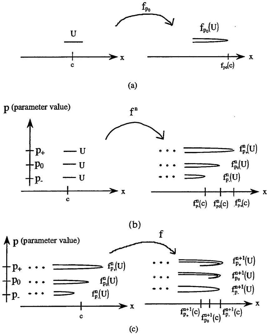
Figure 3.1: Figure 3.1(a) illustrates how neighborhoods near a turning point get folded. (b) shows what might happen for three different parameter values, p_- < p_0 < p_+ . The images of neighborhoods near the critical point tend to get offset each from other so that the neighborhoods for certain parameters (eg., p_+ ) may begin to lead while other parameters (eg., p_- ) lag behind. Lagging parameters have difficulty shadowing leading parameters. (c) shows how neighborhoods can get refolded on each other as a result of a subsequent encounter with a turning point, allowing lagging parameters to “catch up,” so that they are able to shadow parameter values that normally lead.
