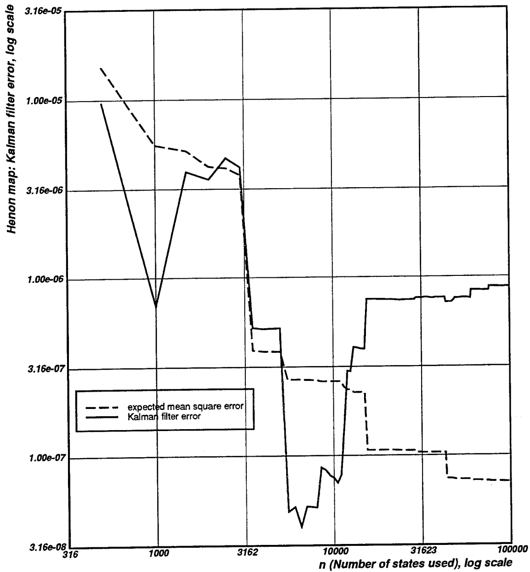
Figure 6.8: This graph depicts the performance of the Kalman filter in estimating parameter a for one sequence of noisy state data from the Henon map for a = 1.4 and b = 0.3 . The data was generated using the initial condition, (x_0, y_0) = (.633135448, 18940634) , which is very close to the attractor.
