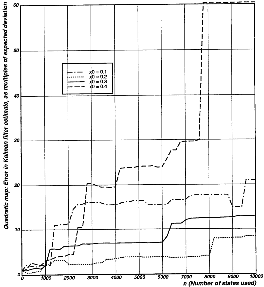
Figure 6.2: This figure shows results for applying the square root extended Kalman filter to estimating the parameters of the quadratic map with p = 3.9 . Each trace represents the average ratio of the actual parameter estimate error to the estimated mean square error as calculated by the Kalman filter over 10 different trials. The different traces represent experiments based on orbits with different initial conditions. Note how the error jumps up to levels on the order of 10 or higher, indicating divergence.
