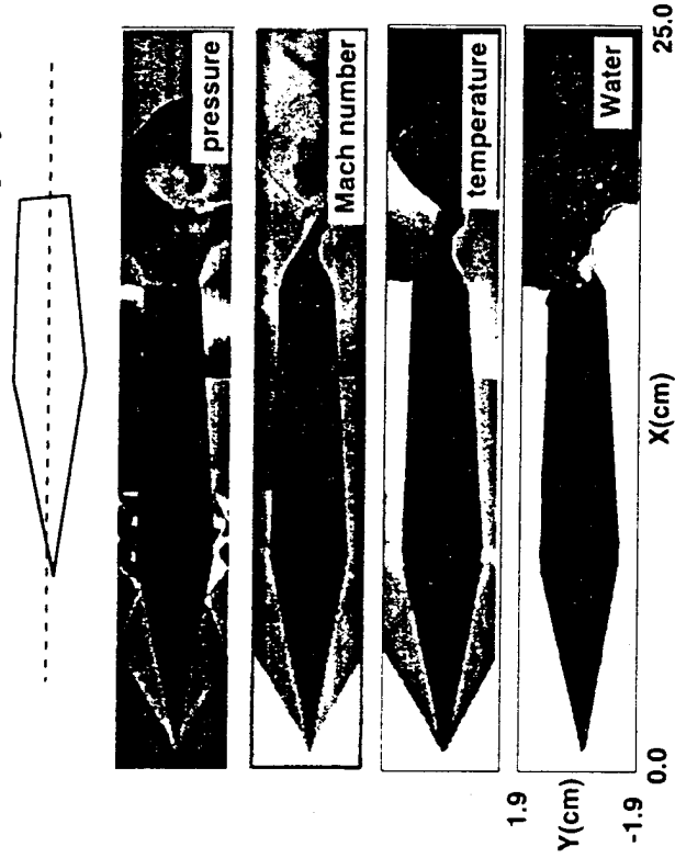
rotated projectile
