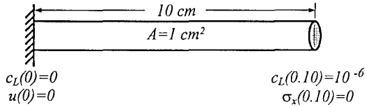
Figure 3: The rod geometry and boundary conditions for Case 1a.
