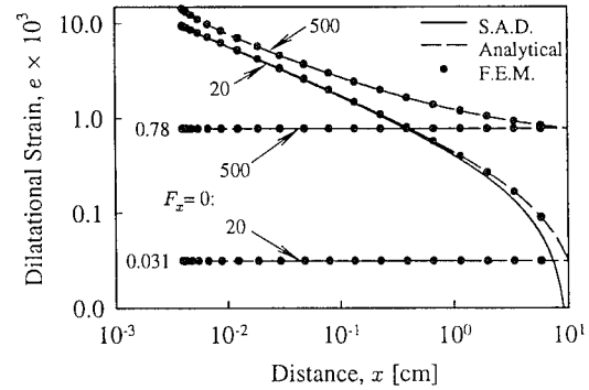
Figure 15: Dilatational strain for Case 3 using the fully coupled and SAD theories.
