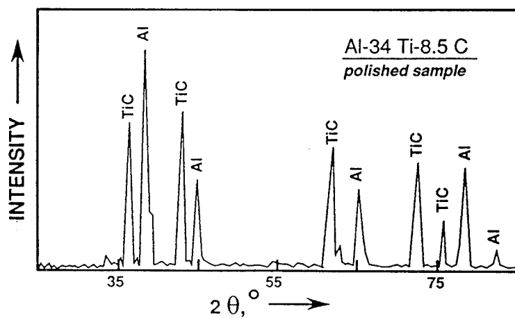
Figure 2-43 X-ray diffraction patterns of the SHS-processed TiC/Al composite: (a) as-received; (b) after polishing.
