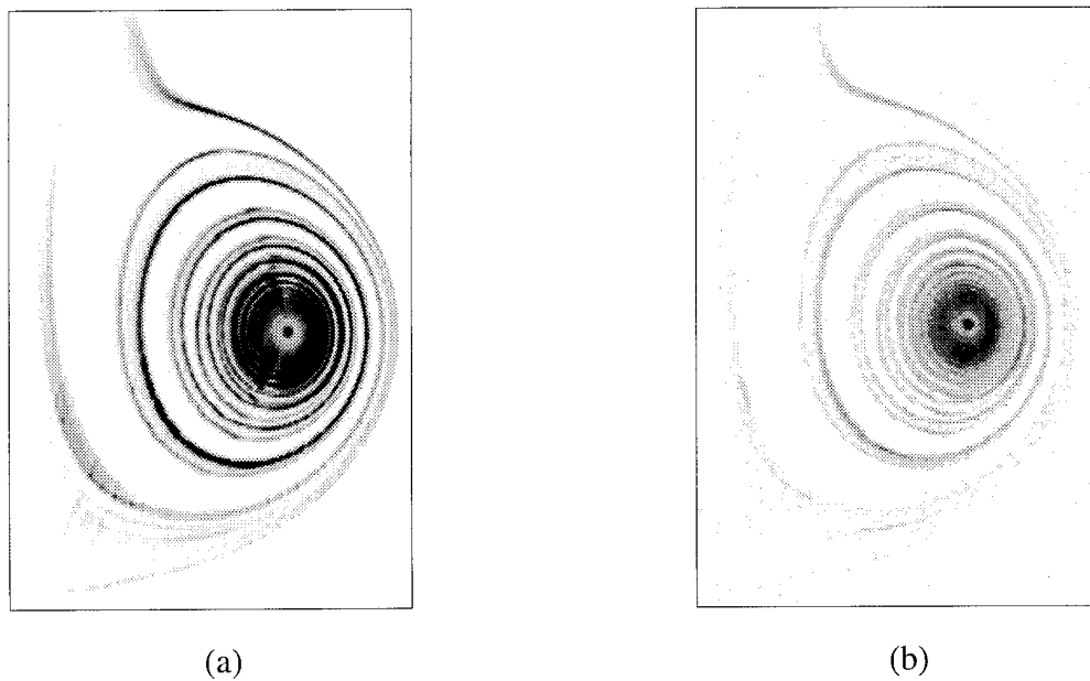
Figure 11. The chemically reacting interface between a vortex ring and the ambient fluid. (a) was imaged 20 \mu sec after tagging with a laser sheet; (b) shows the same interfaces 6 msec later.
