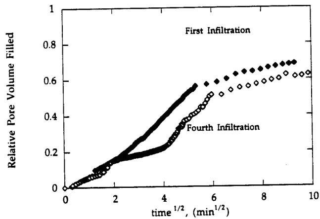
Figure 2 First and fourth infiltration cycle reported as relative pore volume filled as a function of \text{time}^{1/2} for the case of Mullite precursor infiltration into a porous, alumina powder compact.
