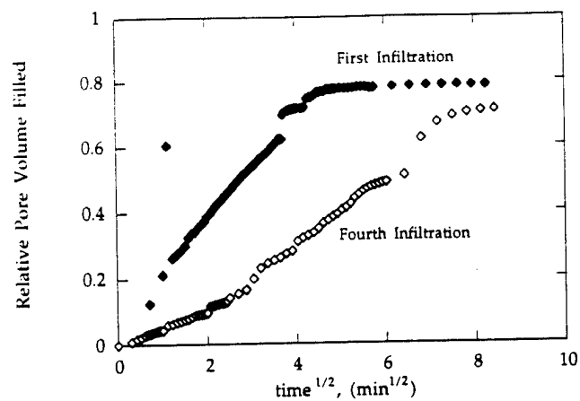
Figure 1 First and fourth infiltration cycle reported as relative pore volume filled as a function of \text{time}^{1/2} for the case of \text{Zr(4Y)O}_2 precursor infiltration into a porous, alumina powder compact.
