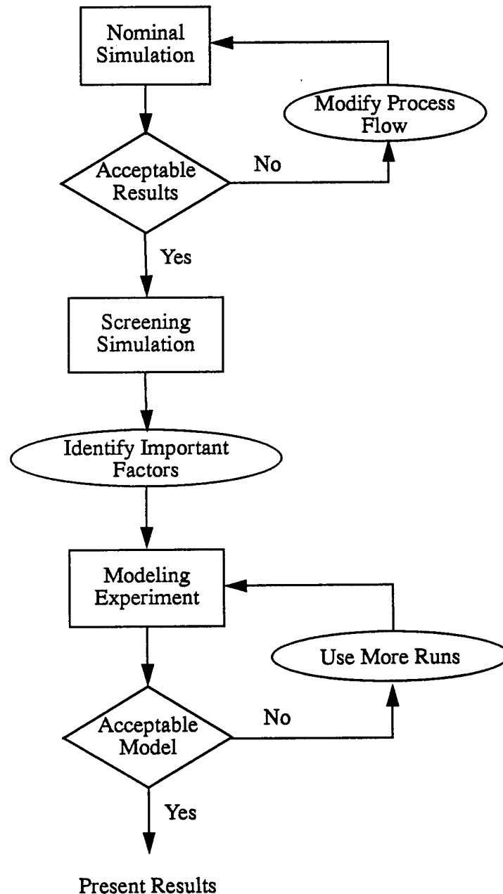
Figure 4-10: Illustration of STADIUM's Statistical Methodology
