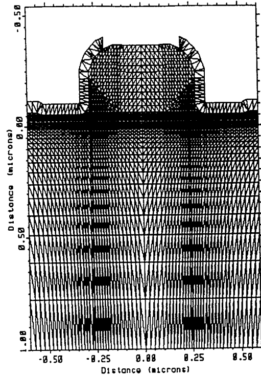
FIGURE 7. Simulation Grid
