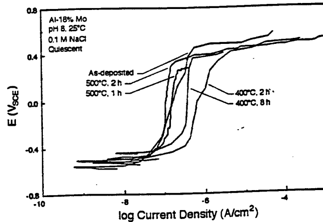
FIGURE 5. Anodic polarization response of Al-18% Mo alloy before and after heat treatment at 400°C for 2 h and 8 h and at 500°C for 1 h and 2 h, polarized in quiescent 0.1 M NaCl at pH 8, 25°C.
