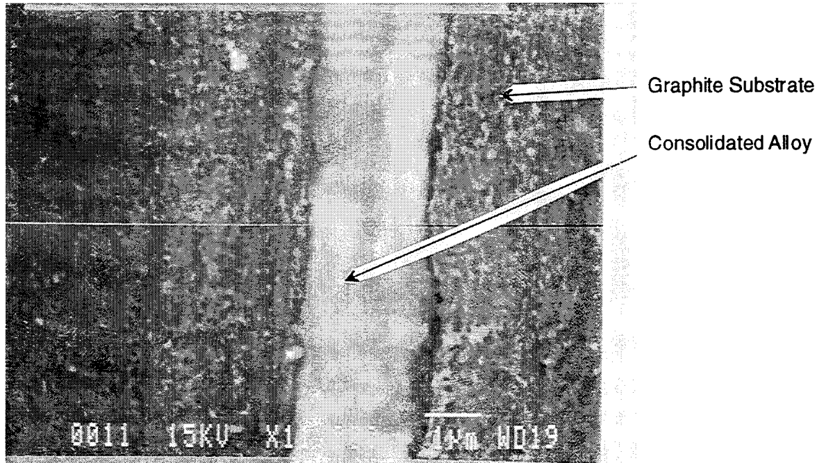
Figure 4-64. HIP specimen made up of two Al-18Mo thin-film alloys in contact with each other after successful consolidation by hot isostatic pressing (HIPing). HIP Parameters: 450^\circ\text{C} , 69 MPa, 60 minutes
