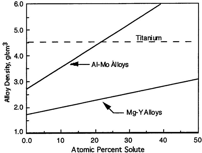
Figure 4-25. Density for Al-Mo and Mg-Y alloys showing maximum solute concentration for the alloy to remain lighter than titanium.
