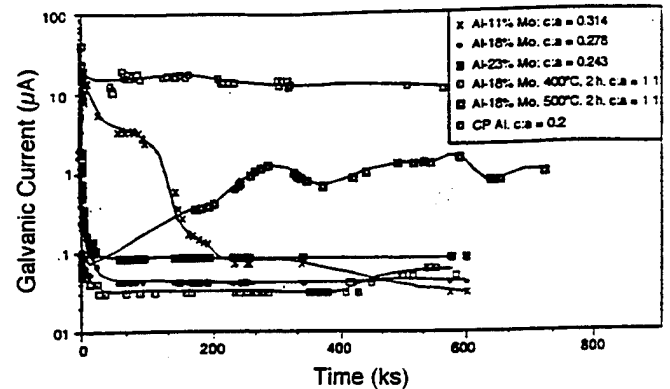
FIGURE 10. Galvanic current for commercially pure (CP) Al and Al-Mo alloys (as-deposited and HT) coupled to P75 Gr fibers in quiescent 0.1 M NaCl at pH 8, 25°C.
