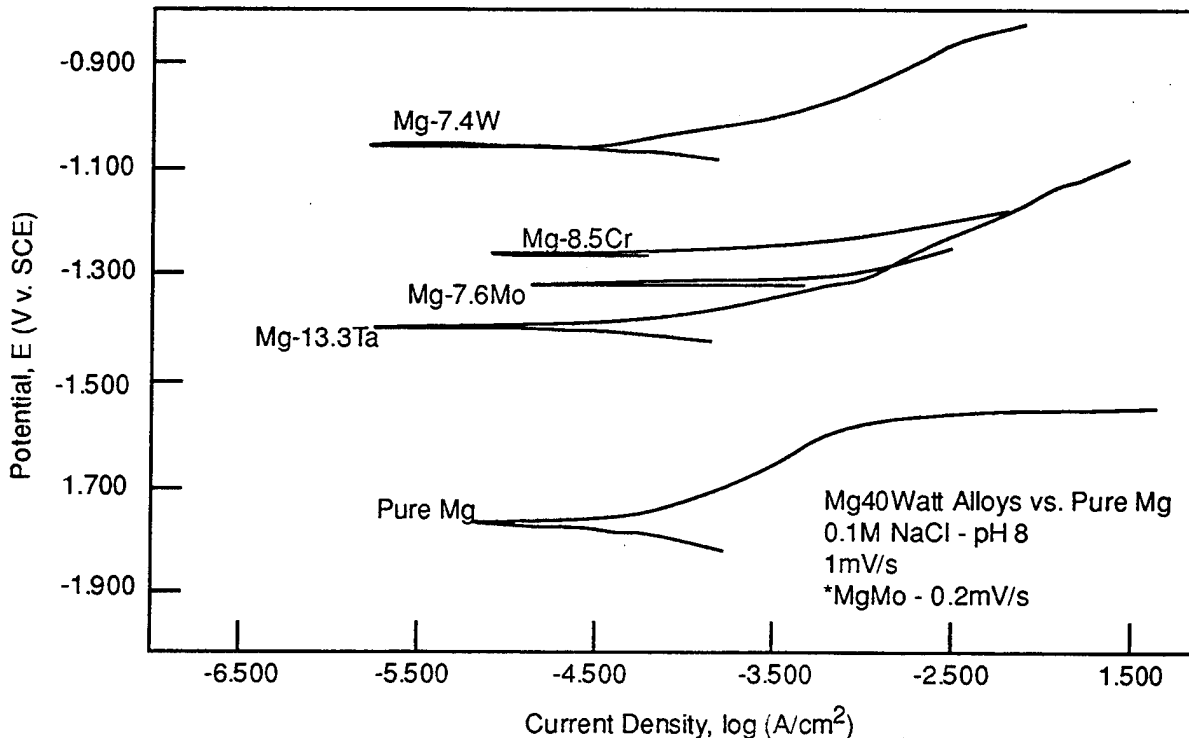
Figure 4-14 Anodic polarization behavior for the highest concentration Mg Alloys generated at a scan rate of 0.2 mV/s in 0.1 M NaCl.
