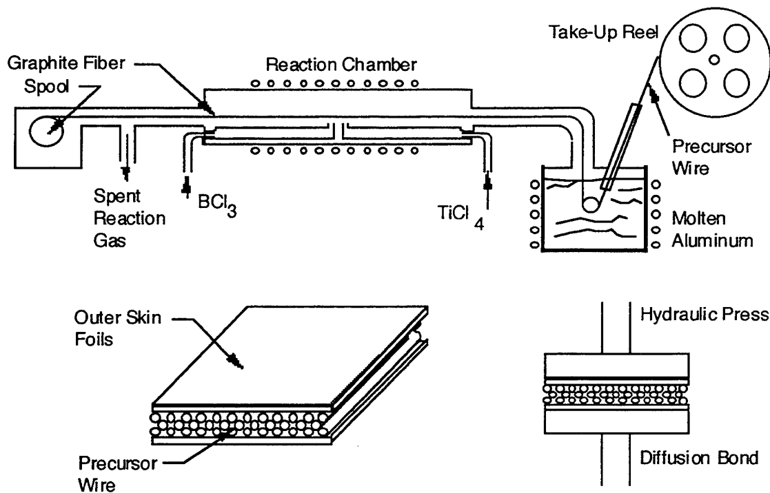
Figure 2-1. Schematic of the liquid metal infiltration process for the production of a Gr/Al composite showing (a) deposition of TiB_2 on the graphite Fibers and directly passing through molten aluminum to create composite wires, (b) lay-up of the composite wires between facesheet foils, and (c) diffusion bonding of the composite.
