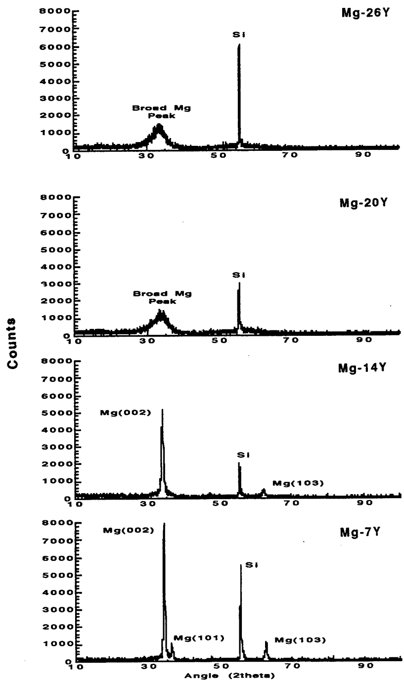
Figure 1. XRD patterns for four of the Mg-Y alloys. Solute concentration decreases moving down the Figure.
