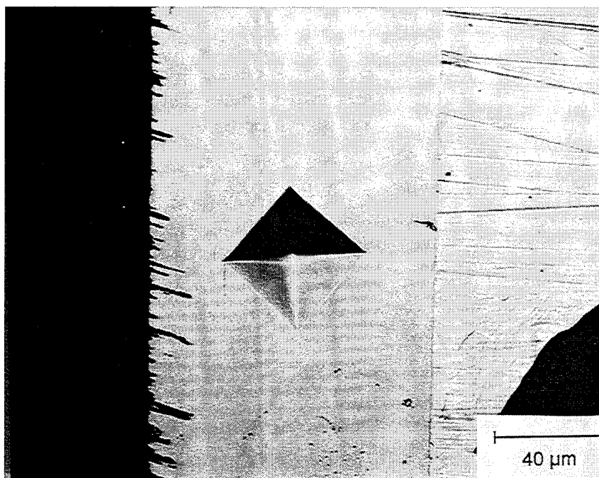
Figure 4-53. Vickers Hardness (Diamond Pyramid Indentation) from a 650 g Load Showing Cracks Propagating From Diamond Tip Parallel To Substrate Interface.
