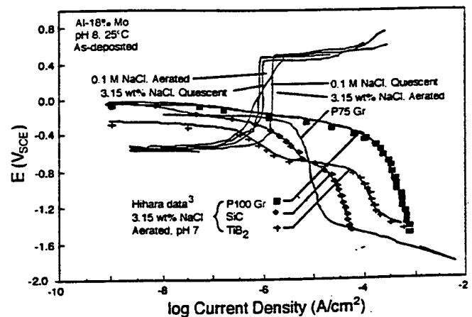
FIGURE 11. Anodic polarization response of Al-18% Mo tested in quiescent 0.1 M and 0.55 M NaCl at pH 8, 25°C superimposed with P75 cathodic curve and cathodic data for P100, SiC, and TiB 2 from Hihara and Latanision. 3
