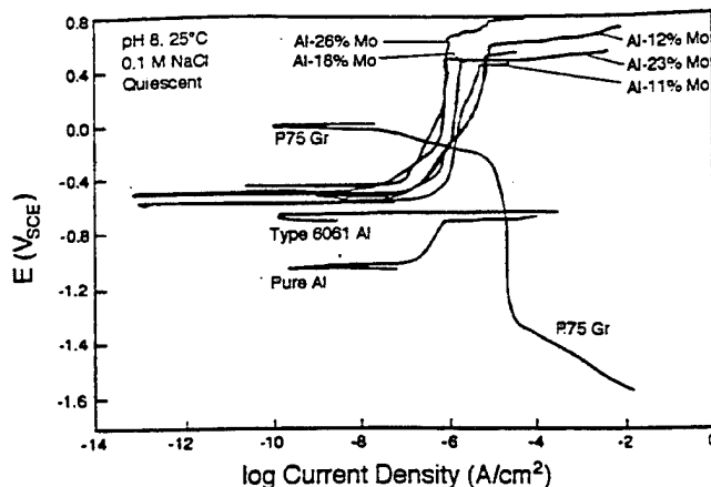
FIGURE 7. Galvanic diagram showing the anodic curve of pure sputtered Al, wrought type 6061 Al, and various sputtered Al-Mo alloys combined with the cathodic curve for an equal area of P75 Gr fibers, tested in quiescent 0.1 M NaCl at pH 8, 25°C.
