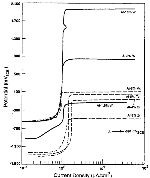
FIGURE 1. Anodic polarization behavior for nonequilibrium Al alloys in aerated 0.1 M KCl compared to spontaneous pitting potential of pure Al ( -691 \text{ mV}_{SCE} ) at 0.167 mV/s. (Reprinted with permission, J. Electrochem. Soc. 138 [1991]: p. 3,292).
