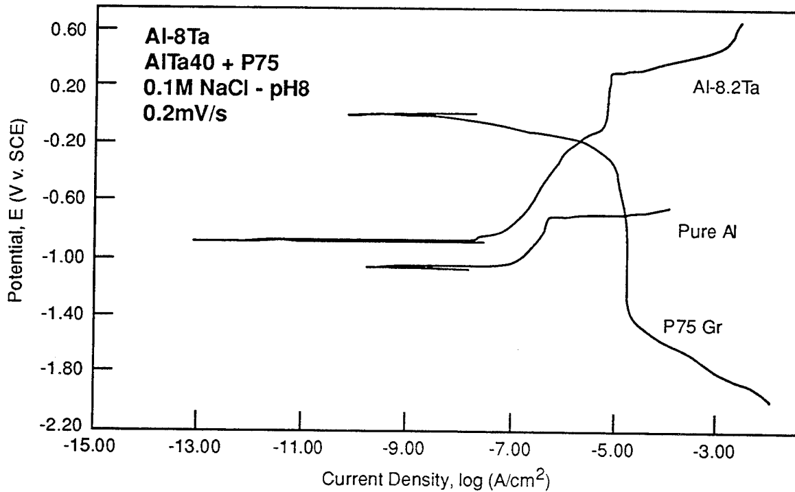
Figure 4-13. Galvanic diagrams for pure Al and Al-8Ta coupled (individually) to P75 graphite in 0.1M NaCl.
