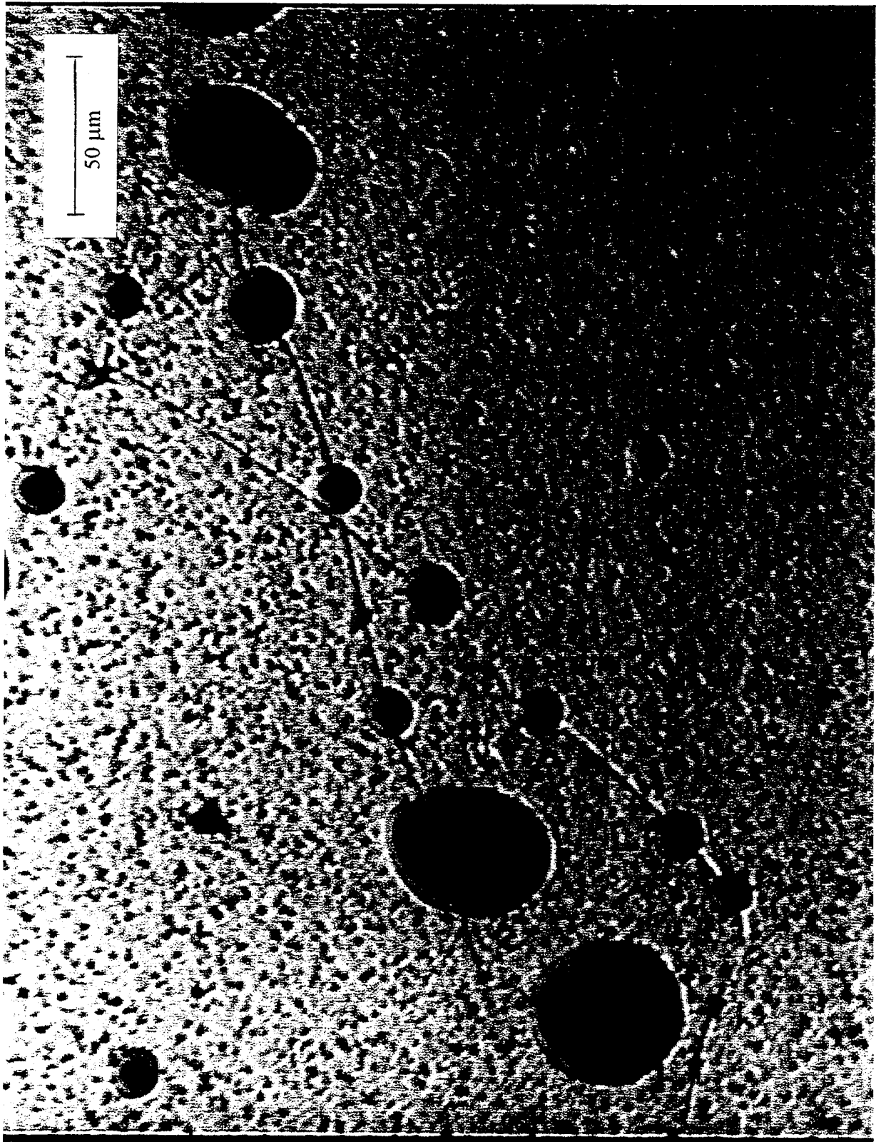
Figure 8. In-situ scanning laser micrograph showing the formation of pits along scratches in a thin film alloy during polarization in 0.1 M NaCl.
