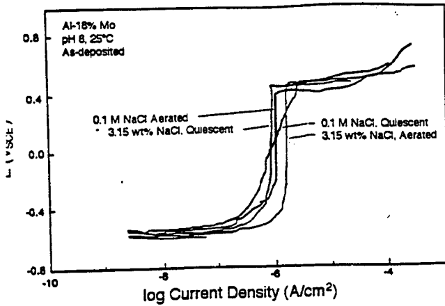
FIGURE 3. Anodic polarization response of Al-18% Mo used for detailed heat treatment studies in quiescent and aerated 0.1 M and 3.15 wt% (0.55 M) NaCl at pH 8, 25°C.
