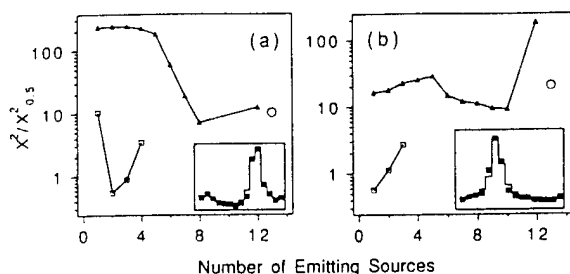
Fig. 5. \chi^2 test of the different localized plasma domains. \chi^2/\chi_{0.5}^2 is plotted as a function of the number of emitting domains and inserts show the best fit, e.g., for the case when \chi^2/\chi_{0.5}^2 is a minimum. The following plasma representations are used: the point sources ( \square ); the lump sources on impact with a set of neighboring GM-counters ( \blacktriangle ); and the 13 equal-volume sources ( \circ ). \chi^2 is from comparison of A_{th} and A_{exp} ; \chi_{0.5}^2 is the theoretical value of \chi^2 that would be obtained for a fit with a confidence level of 50%.
