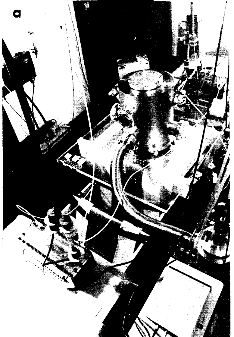
Fig. 4: APF-50 general view. Configuration 1 at right, Configuration 2 at left.
