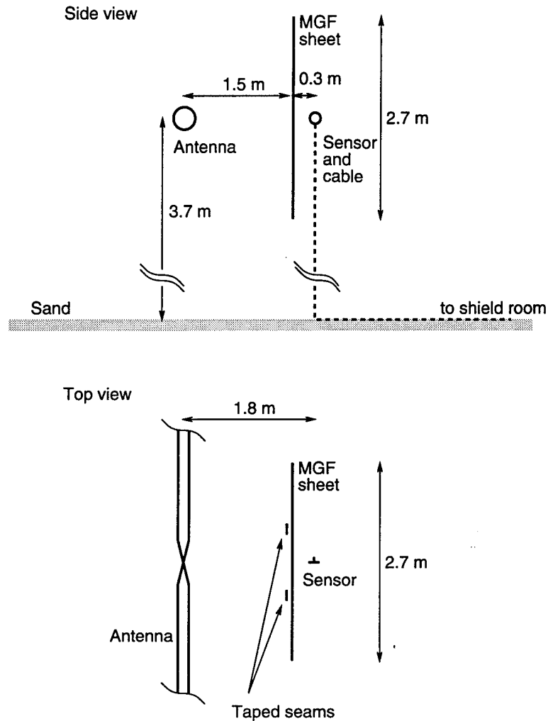
Figure 3. Physical relationship between dipole, MGF sheet, and sensor (drawn to scale).
