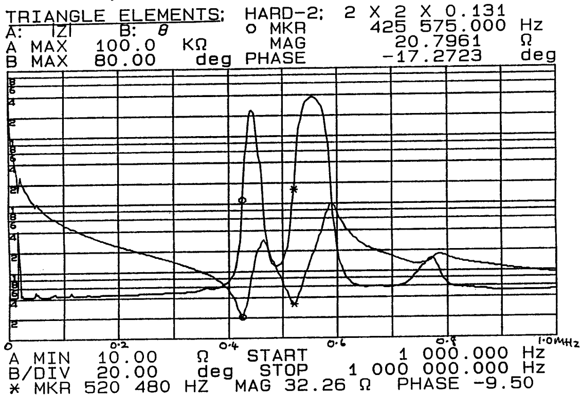
Figure 20: Impedance/frequency characteristics of triangular PZT element array, Shore D-85 polyurethane matrix.
