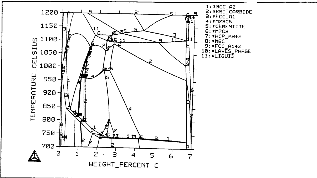
Figure 1: Predicted phase diagram for M50 as a function of temperature and wt%C. Numbered lines outline regions where a particular phase, identified in the key, is expected.
