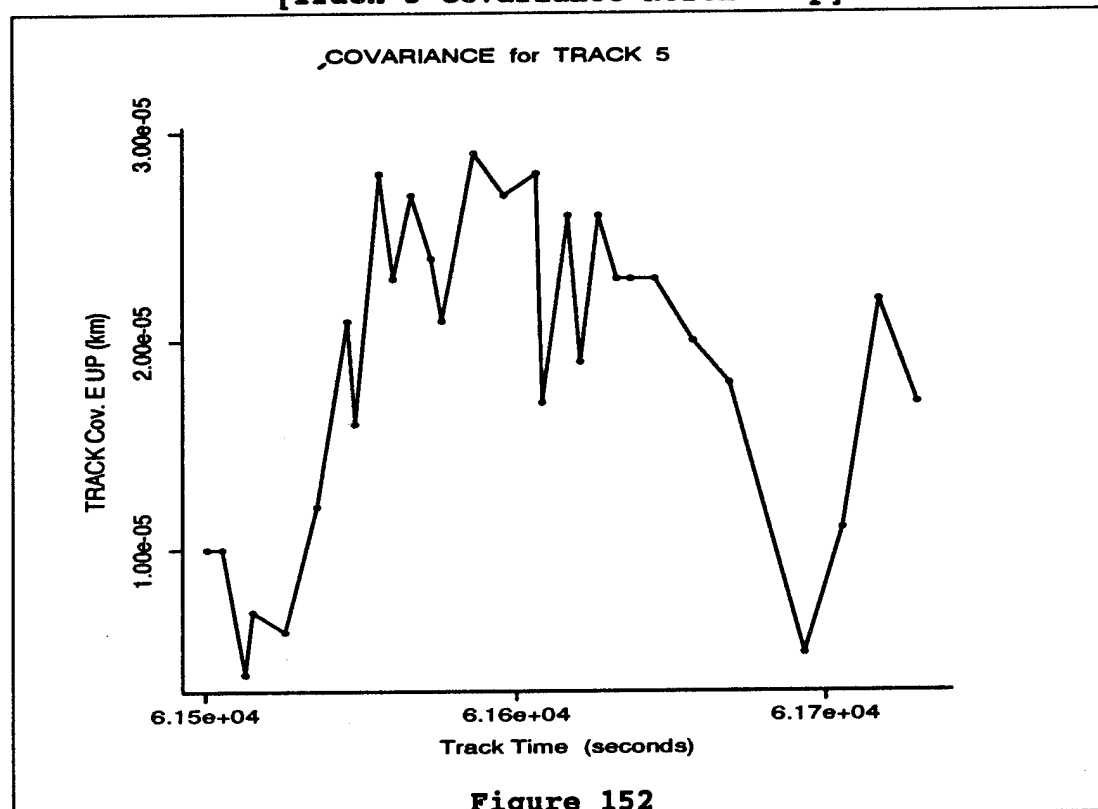
Figure 152 [Track 5 Covariance East - Up]
