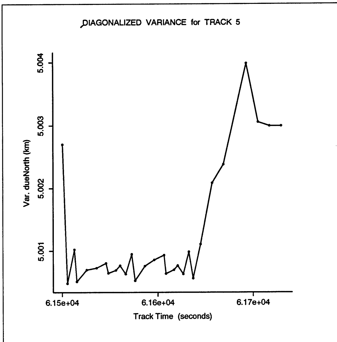
Figure 158 [Track 5 DIAGONALIZED Variance due North]
