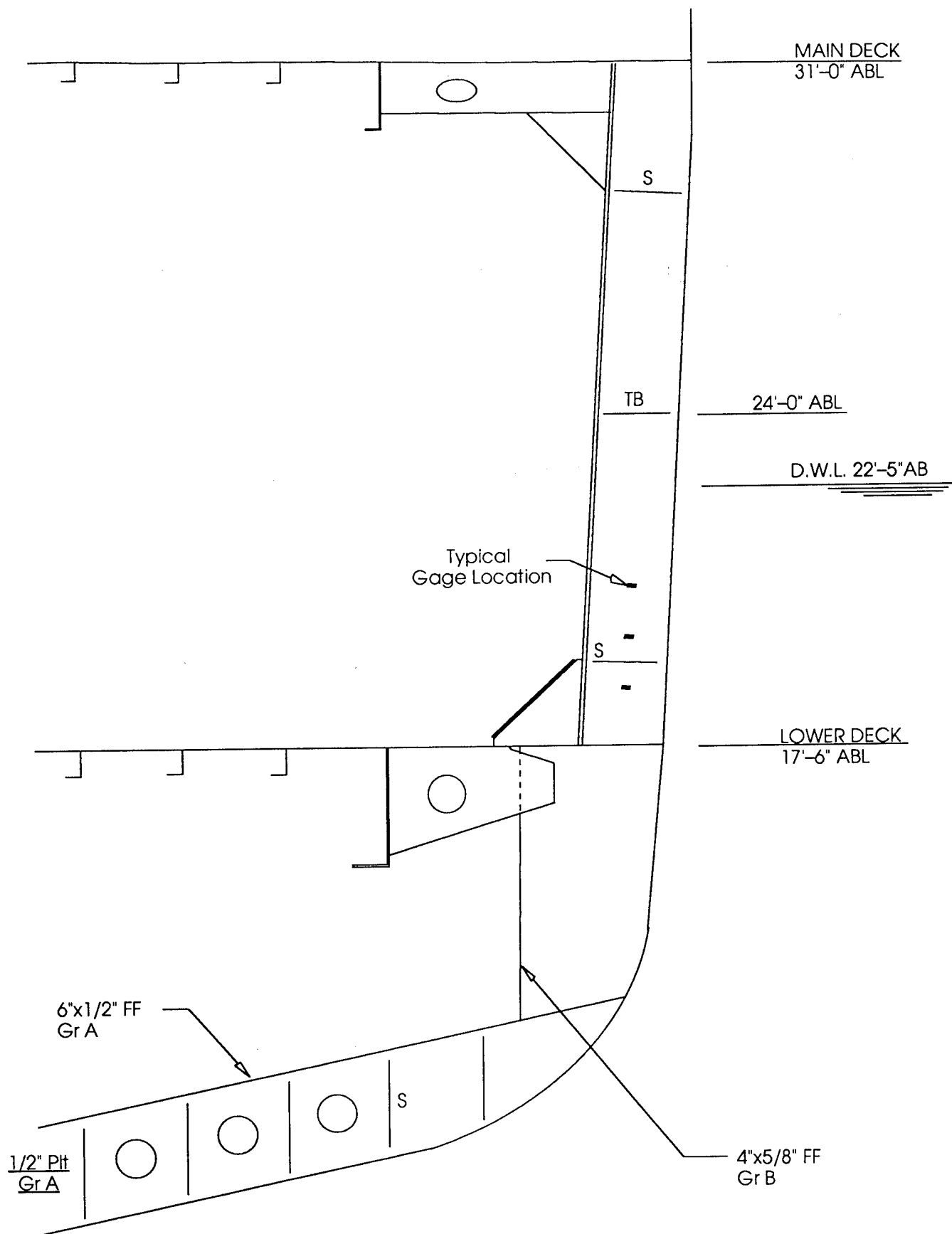
Figure 5. Transverse frame 39.
