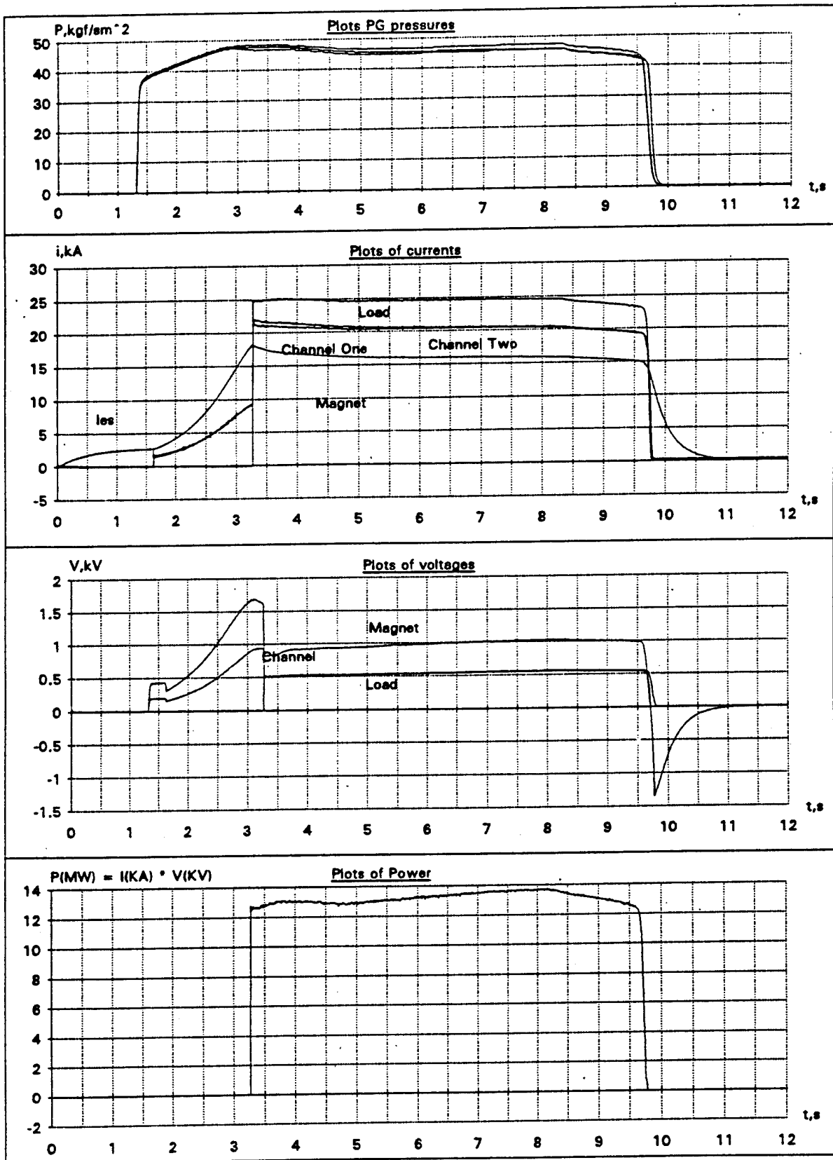
Figure 63 Performance Results from Acceptance Test No. 2
