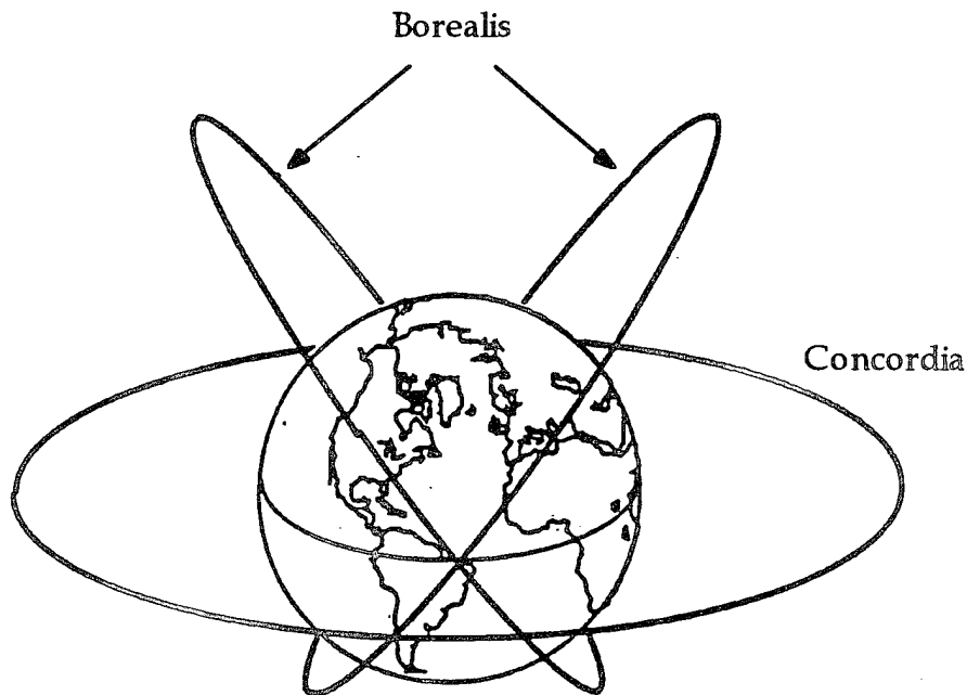
Figure 2-7 Ellipso Constellation
