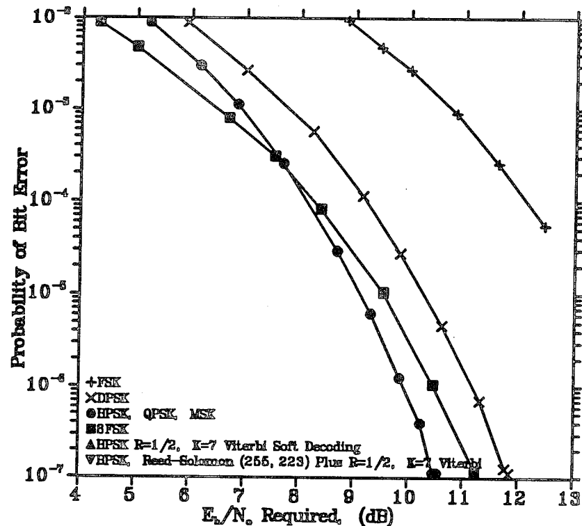
Figure 5-8 E_b/N_0 vs BER relationships [Davies, 1992].
