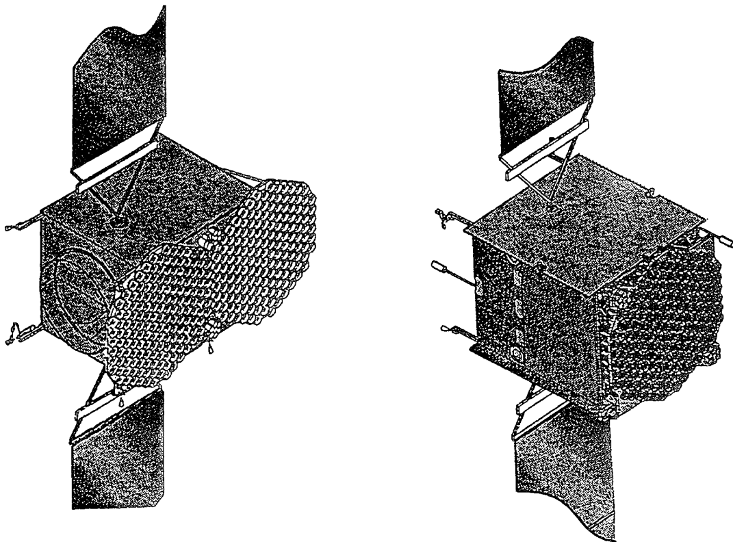
Figure 2-9 Possible Inmarsat-P Antenna Configurations [Jurkiewicz, 1995].
