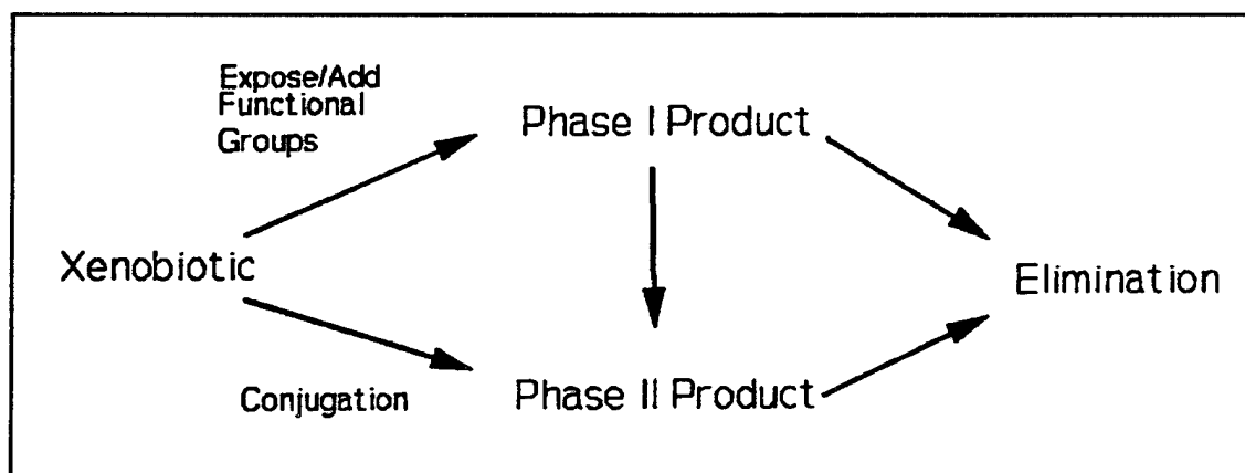
Figure 1. Schematic of phase I and II metabolism
