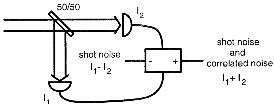
Figure 3.1: Homodyne Detector
