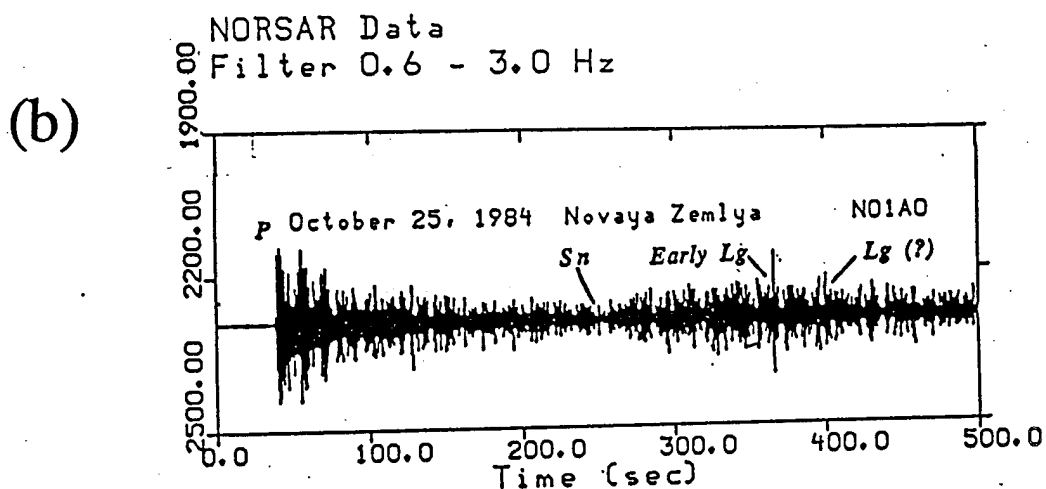
Figure 19-(a). Comparison of the ARCESS FRAO trace of the December 4, 1988 explosion with the NORSAR NO1A0 recording of the September 4, 1972 Kola Peninsula explosion. (b) The NORSAR NO1A0 trace of the October 25, 1984 explosion.
