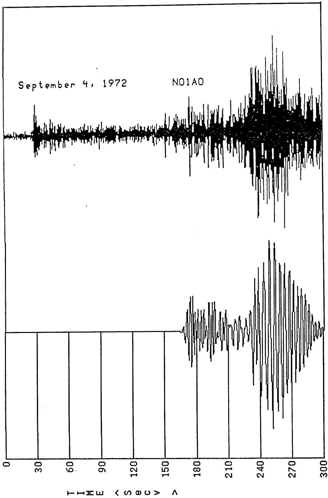
Figure 21-(b). Comparison of the numerical result and the real data for the NORSAR NO1A0 of the September 4, 1972 Kola Peninsula explosion.
