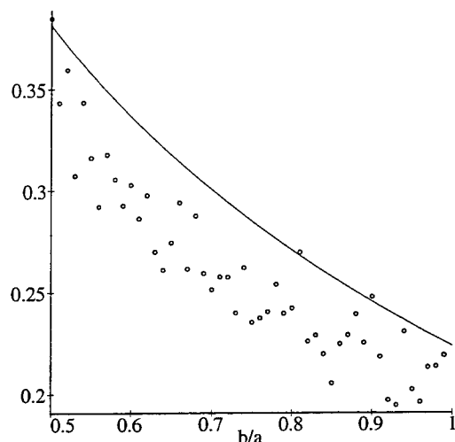
Figure 5-20: Centroid error for an elliptical fiducial with a radius of 10. The error is expressed in pixels and b/a is the ratio of minor and major axis.
