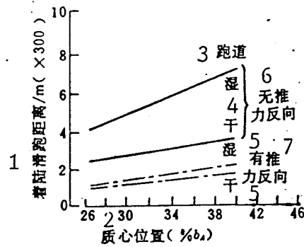
Fig. 7. Effect on landing roll distance of thrust reversal KEY: 1 - landing roll distance 2 - position of mass center 3 - runway 4 - wet 5 - dry 6 - without thrust reversal 7 - with thrust reversal
