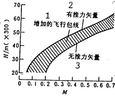
Fig. 5. Effect on flight due to thrust vectoring KEY: 1 - expanded flight envelope 2 - with thrust vectoring 3 - without thrust vectoring
