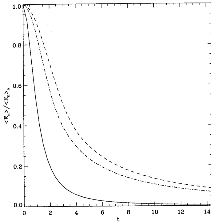
Figure 3.8: Normalized energy decay for an inner-core asymmetry of the AB model (top) and the GSM model (bottom). The GSM curves are the energy decay for: n = 2 (dash), n = 3 (dot dash), and the limiting energy decay calculated from the effective shear of the Rankine vortex (solid). The characteristic time scale for both plots is roughly two circulation times.
