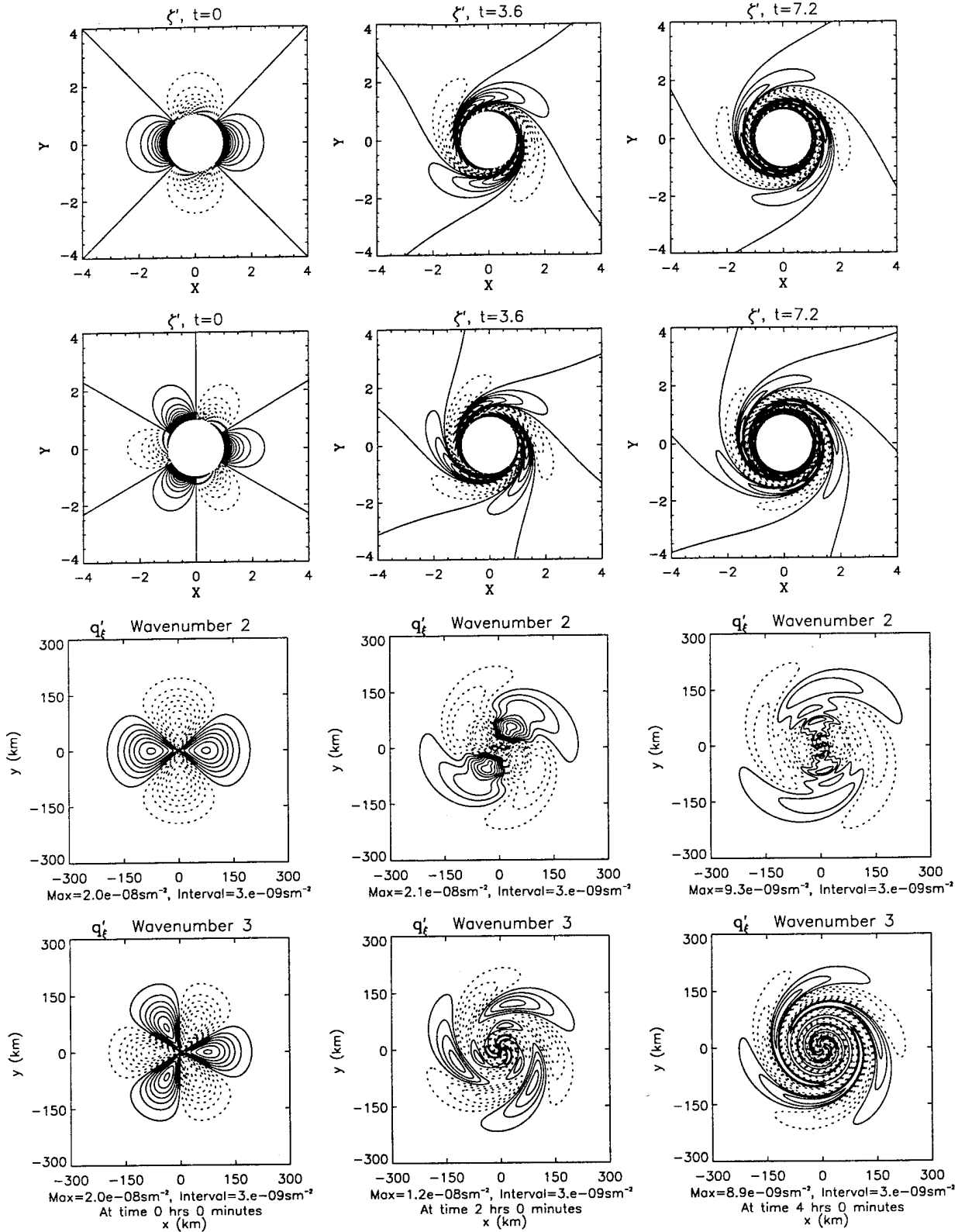
Figure 3.5: Perturbation vorticity, \zeta' , in the GSM model for the bounded vortex using a contour interval of 6.90 \times 10^{-2} (first two rows). The perturbation potential vorticity, q'_\xi , in the AB model (last two rows). Columns correspond to roughly 0, 1/2, and 1 circulation times in both models. The horizontal domain corresponds to four RMW units in both models.
