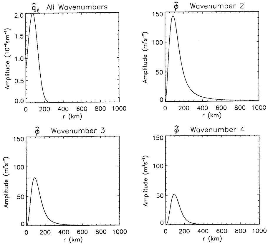
Figure 3.4: Radial profiles of initial |\hat{q}_\epsilon| (same for all wavenumbers), and calculated |\hat{\phi}| for wavenumbers two through four. Again note the decreasing |\hat{\phi}| with increasing wavenumber.
