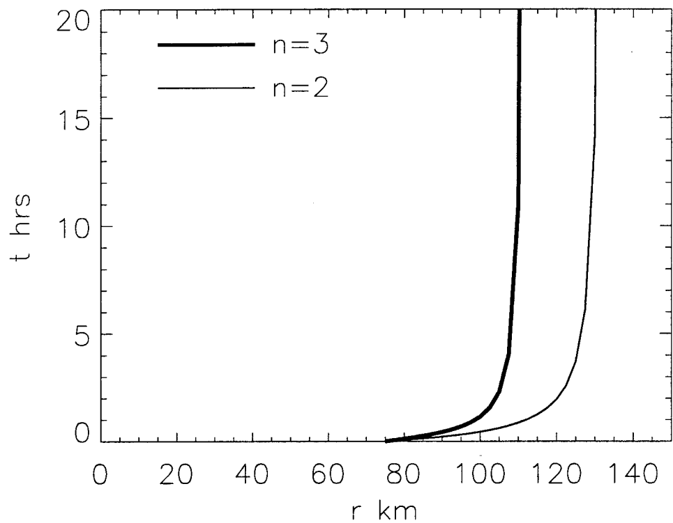
Figure 5.4: WKB radial wave-packet trajectories for wavenumbers two and three calculated by integrating the expression for C_{gr} using the AB benchmark vortex. The top panel shows results using r_o = 200 km, k_o = 1/RMW , while the bottom panel uses r_o = 75 km, k_o = 1.5/RMW .
