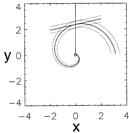
Figure 5.3: Schematic of a local plane-wave approximation to a trailing spiral in the WKB formulation. The solid line represents the wave crest and the dashed lines represent neighboring wave troughs. The x and y scales are in terms of RMW units.
