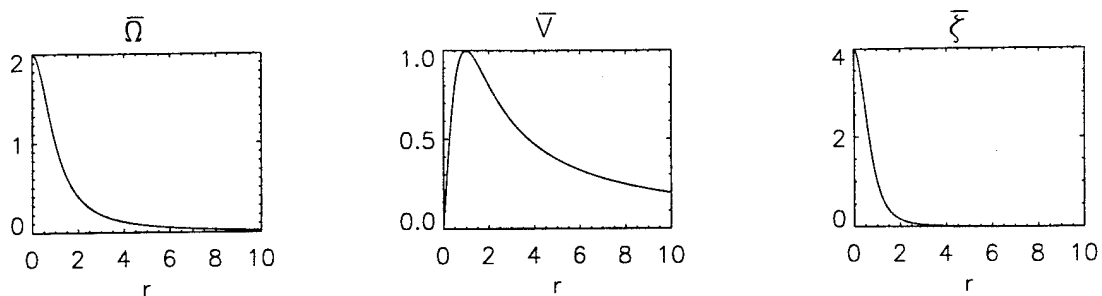
Figure 4.5: The non-dimensional basic state vortex used in the exact solution: \bar{\Omega} = 2/(1+r^2) , \bar{v} = r\bar{\Omega} , \bar{\eta} = \bar{\Omega} + d\bar{v}/dr . The model domain is of length 40, but only the inner 10 units are shown. Although this swirl profile falls off significantly faster than the benchmark vortex of the AB model, it is nevertheless stable to exponential disturbances.
