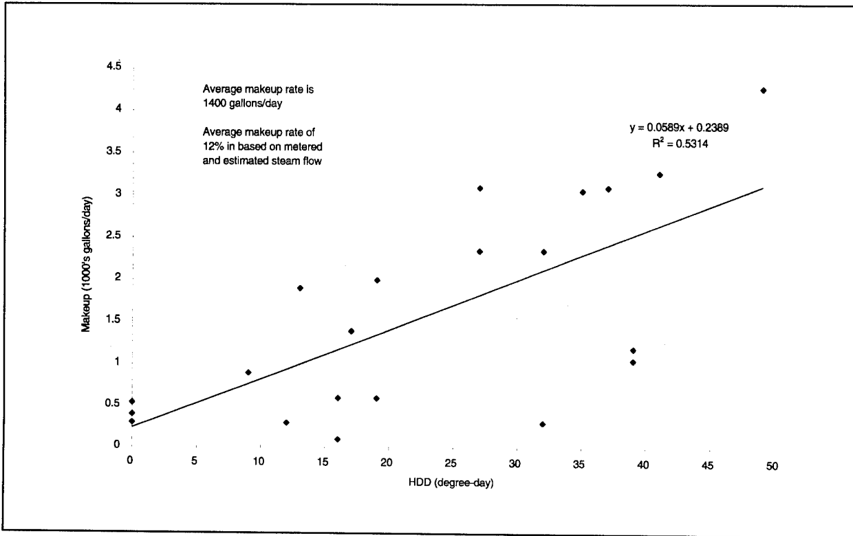
Figure 5. Makeup rate versus heating degree-days for CHP 5324.
