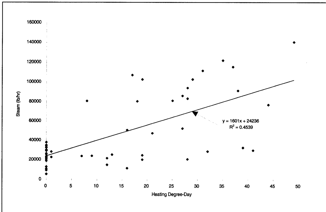
Figure 11. Total steam distribution system production, CY92.
