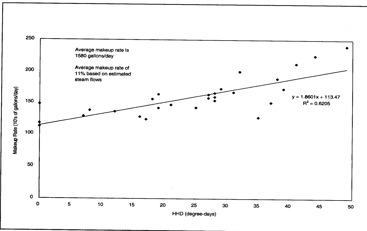
Figure 6. Makeup rate versus heating degree-days for CHP 5426.
