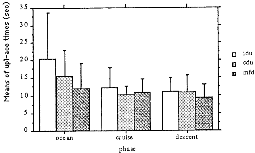
FIGURE 9. UPLINK-ACCEPT TIMES
