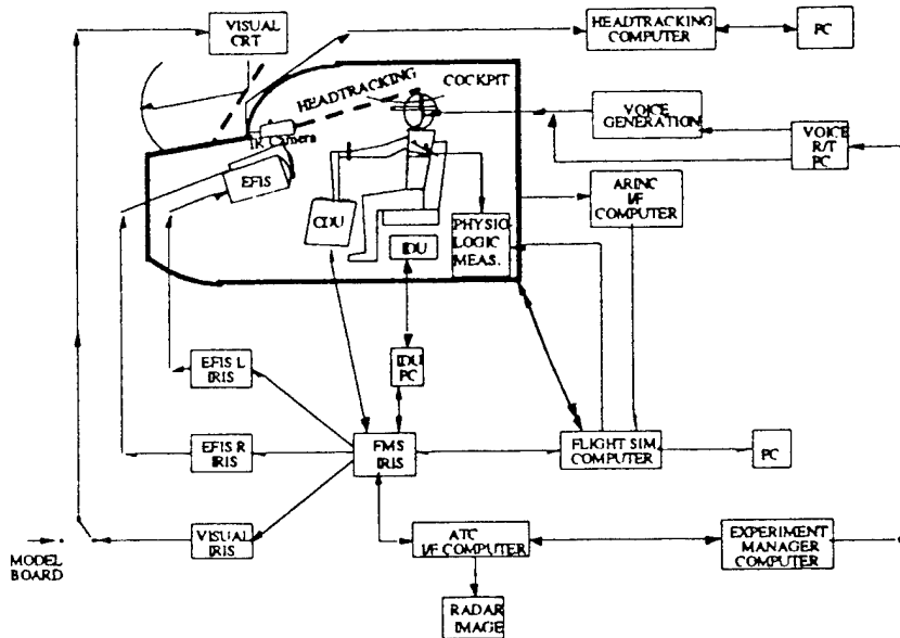
FIGURE 1. FUNCTIONAL DIAGRAM OF THE SIMULATION FACILITIES
