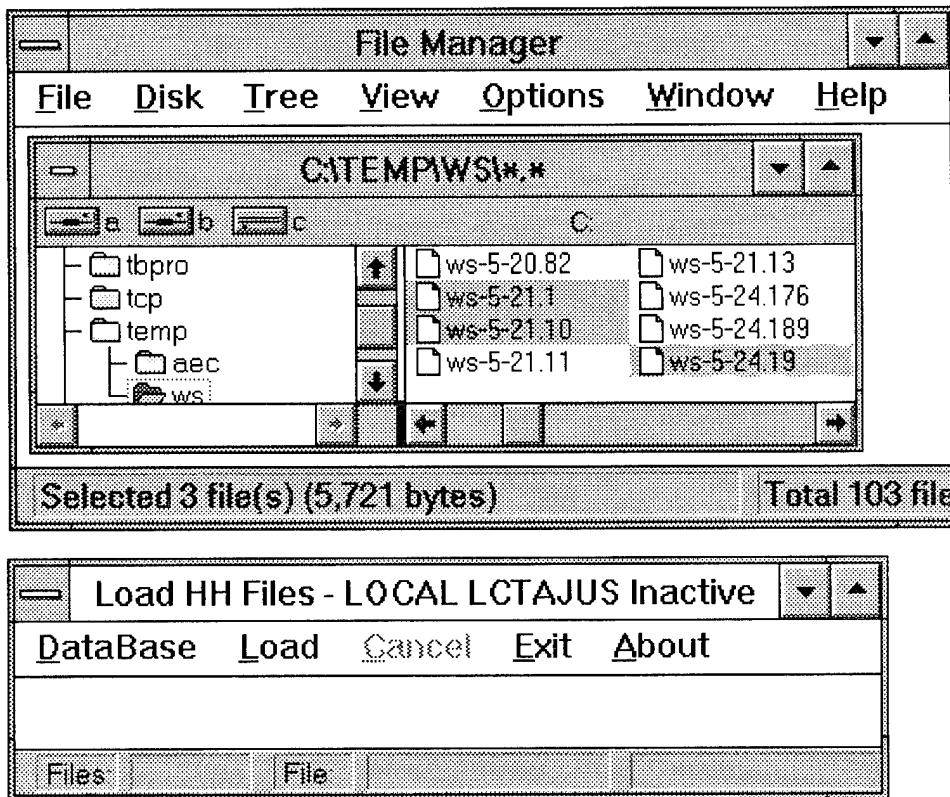
Figure 56. Loading data files by dragging and dropping files from the Windows File Manager into the LCTA Field Data Database Loading program.
