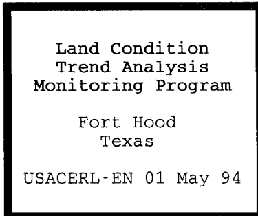
Figure 37. Title window.
