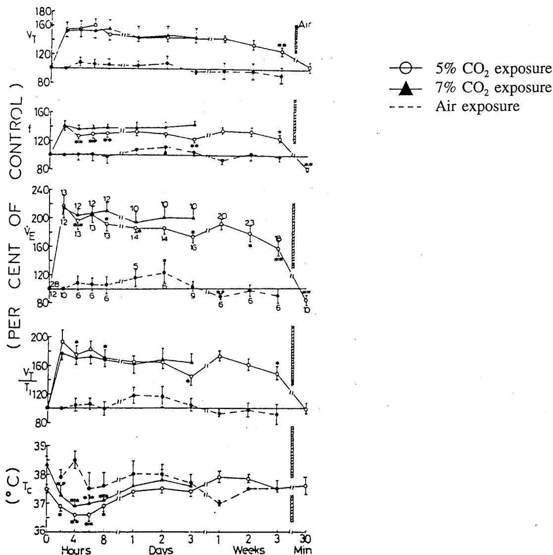
FIGURE 40. VENTILATORY PARAMETERS ( V_T , f , \dot{V}_E , AND V_T/T_I ) PER 100 g BODY WEIGHT, EXPRESSED AS A PERCENTAGE OF BASELINE (AIR BREATHING AT BEGINNING OF STUDY) AND BODY TEMPERATURE ( T_c ) DURING CONTINUOUS 5% AND 7% CARBON DIOXIDE EXPOSURE AND AIR BREATHING (LAI)
