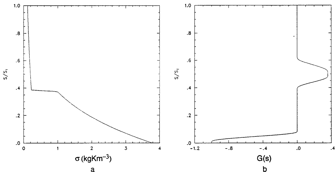
Figure 4.1: Control simulation initial (a) \bar{\sigma}(s) and (b) G(s) profiles.
