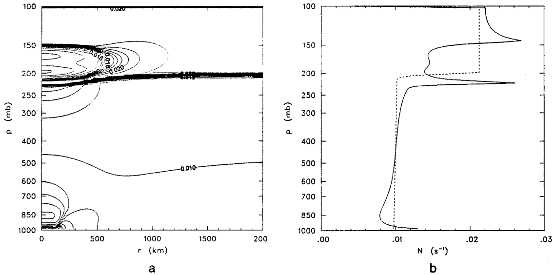
Figure 4.7: Control simulation (a) buoyancy frequency N ( 0.005 s^{-1} contour interval) following the adjustment including the (b) inner (solid) and outer (dashed) boundary profiles. Notice the sharp peaks in N above and below the perturbation.
