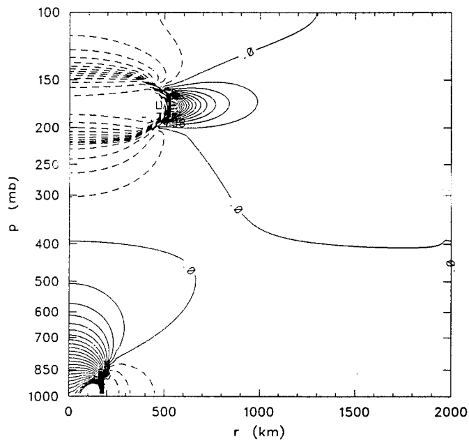
Figure 4.8: Control simulation isentropic relative vorticity \zeta following the adjustment ( 5.0 \times 10^{-6} s^{-1} contour interval).
