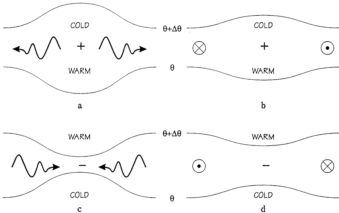
Figure 3.1: (a) Atmosphere perturbed by a mass source “+” with (b) the resulting balanced state. (c) Atmosphere perturbed by a mass sink “-” with (d) the resulting balanced state. The arrows indicate the direction of gravity wave propagation while the circle with a dot in the center denotes flow out of the paper and the circle with an “x” in the center denotes flow into the paper.
