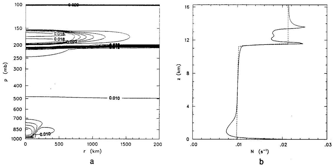
Figure 4.23: Same as Fig. 4.7 except that the perturbation has been moved south to 10^\circ\text{N} .
