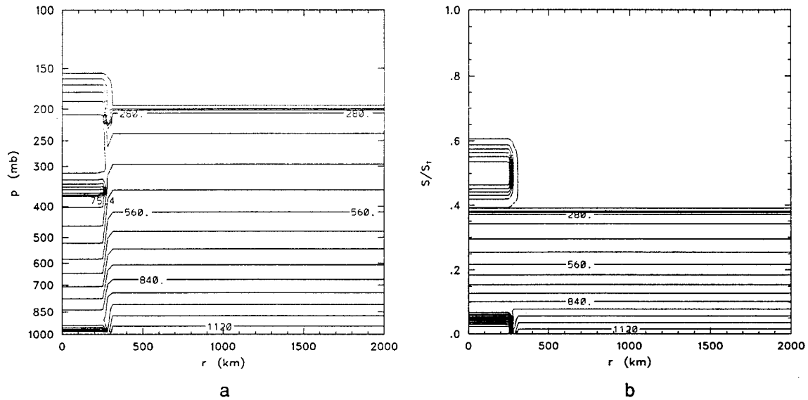
Figure 4.4: Control simulation initial \sigma^* field in (a) isobaric and (b) isentropic coordinates ( 70 \text{ kg km}^{-3} contour interval). Notice the change in the perturbation depth between (a) and (b).
