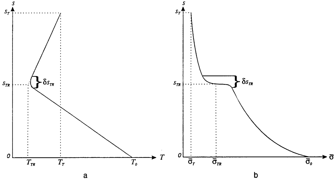
Figure 3.3: Basic state (a) temperature \bar{T}(s) and (b) pseudodensity \bar{\sigma}(s) profiles. \delta s_{TR} is the specific entropy difference over which the tropopause discontinuity is smoothed.
