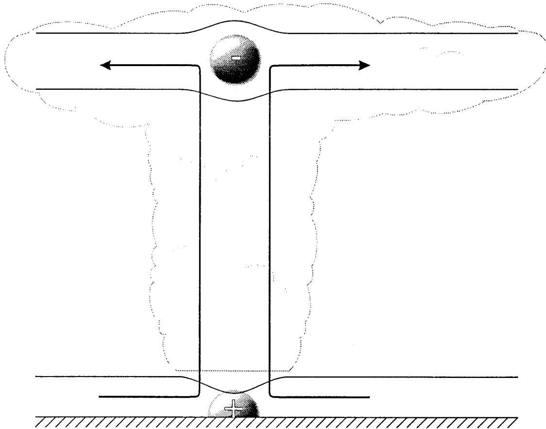
Figure 3.2: Generation of “+” and “-” PV anomalies by moist convection. Horizontal lines represent isentropic surfaces.
