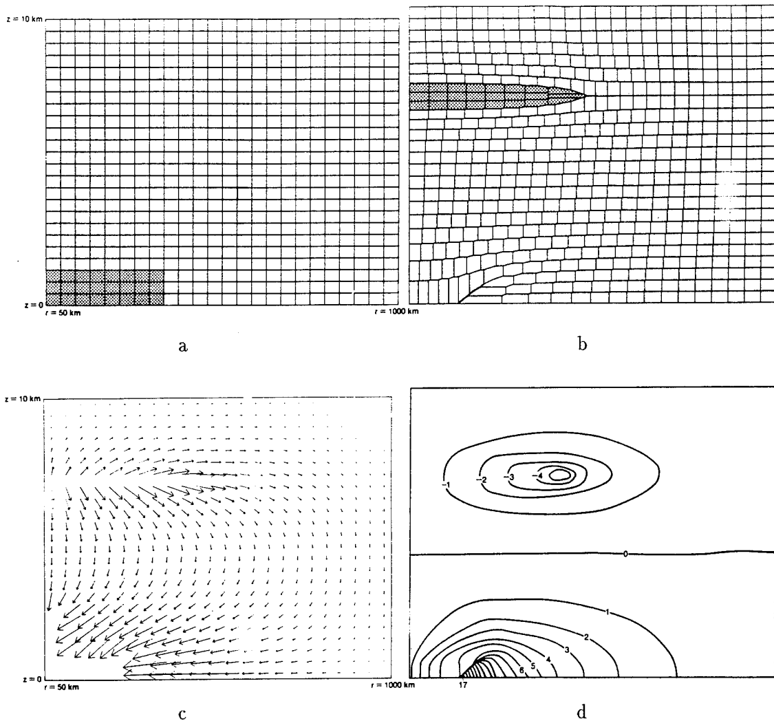
Figure 2.9: Results from an axisymmetric, Lagrangian parcel model. Fields shown are the (a) initial element configuration with shaded area being the positively buoyant elements ( 2.1\text{K} increase in \theta with each element), (b) final element configuration with lens and "eye" wall structure, (c) parcel displacement field, and (d) the balanced tangential velocity ( 1\text{ ms}^{-1} contour interval). Initially, elements in the same horizontal plane have the same potential temperature while elements in the same vertical column have the same angular momentum (From Shutts et al., 1988).
