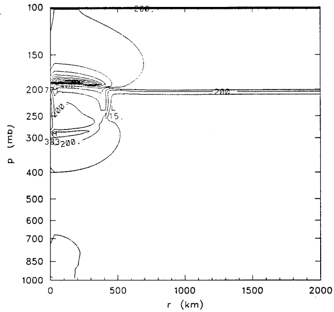
Figure 4.18: Same as Fig. 4.9 except that the 50 mb perturbation is located immediately beneath the tropopause.
