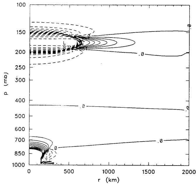
Figure 4.24: Same as Fig. 4.8 except that the perturbation has been moved south to 10^\circ\text{N} .
