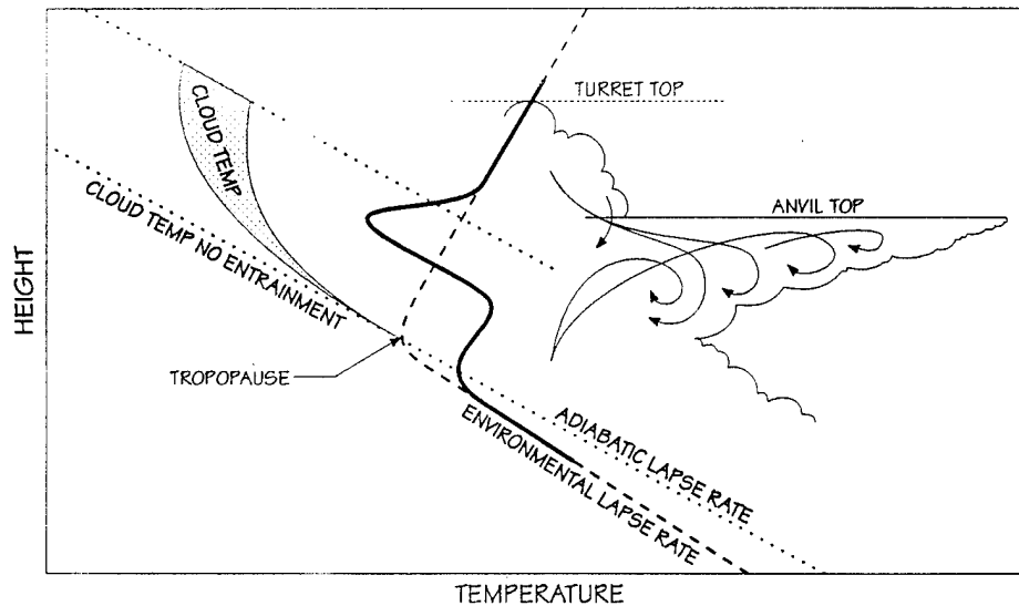
Figure 2.10: Theoretical mechanism for stratospheric anvil formation and its associated temperature distribution (From Danielsen, 1982).
