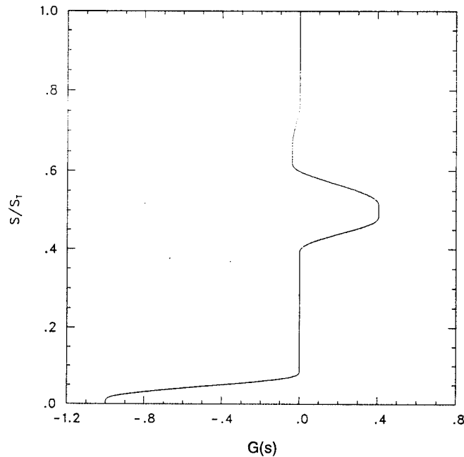
Figure 4.28: Profile of G(s) including an additional mass sink along the top of the outflow.
