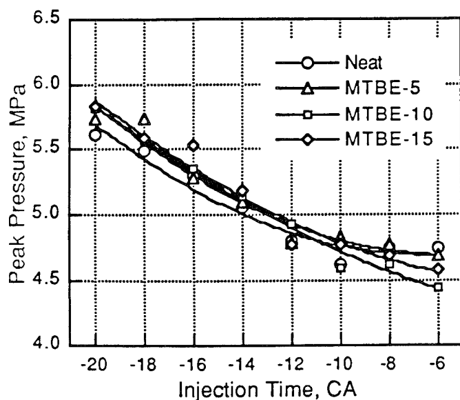
Fig. 2. Peak Cylinder Pressure Obtained with Different Fuels.
