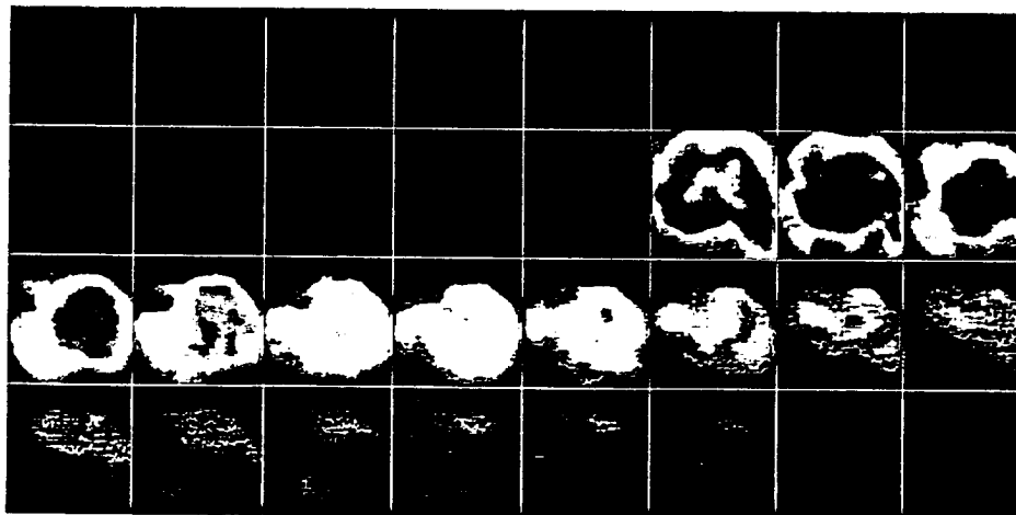
Fig. 6. High-speed Spectral IR Images of a Plume in CI-DI Engine Combustion Chamber in Band of 2.2\text{-}2.5\mu\text{m} for Injection started at (1) 25bTDC; (2) 18bTDC; (3) 12bTDC and (4) 4bTDC.
