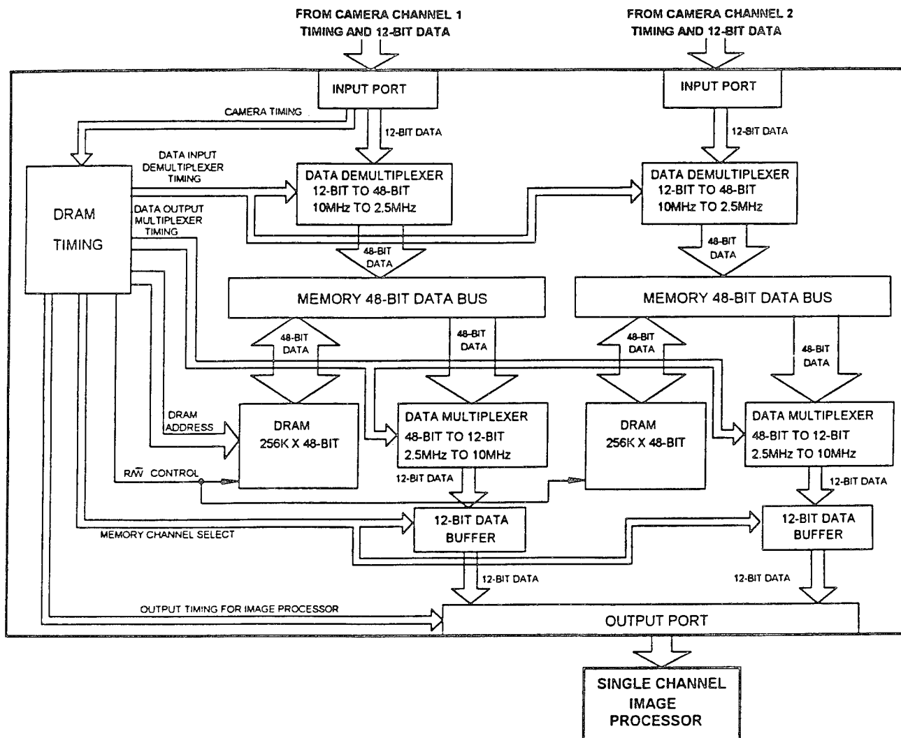
Fig. 4 Block diagram of memory subsystem.
