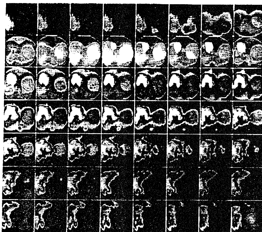
Fig. 7. High-speed Spectral IR Images of In-cylinder Events with a Gasoline-air Mixture near the Stoichiometric (Warm Engine): (A) 2.47 \mu m and (B) 3.43 \mu m.
