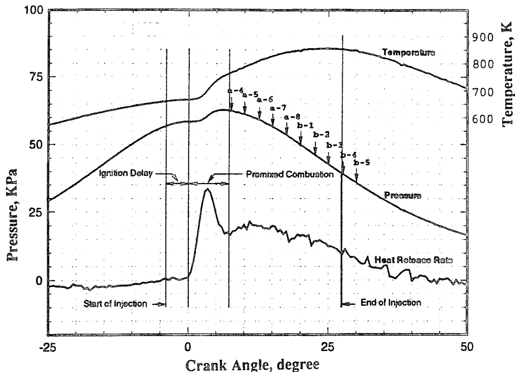
Fig. 1. Pressure-Time (p-t) Measured of Single-Cylinder Engine and Markers to Show Corresponding Imaging Times.
