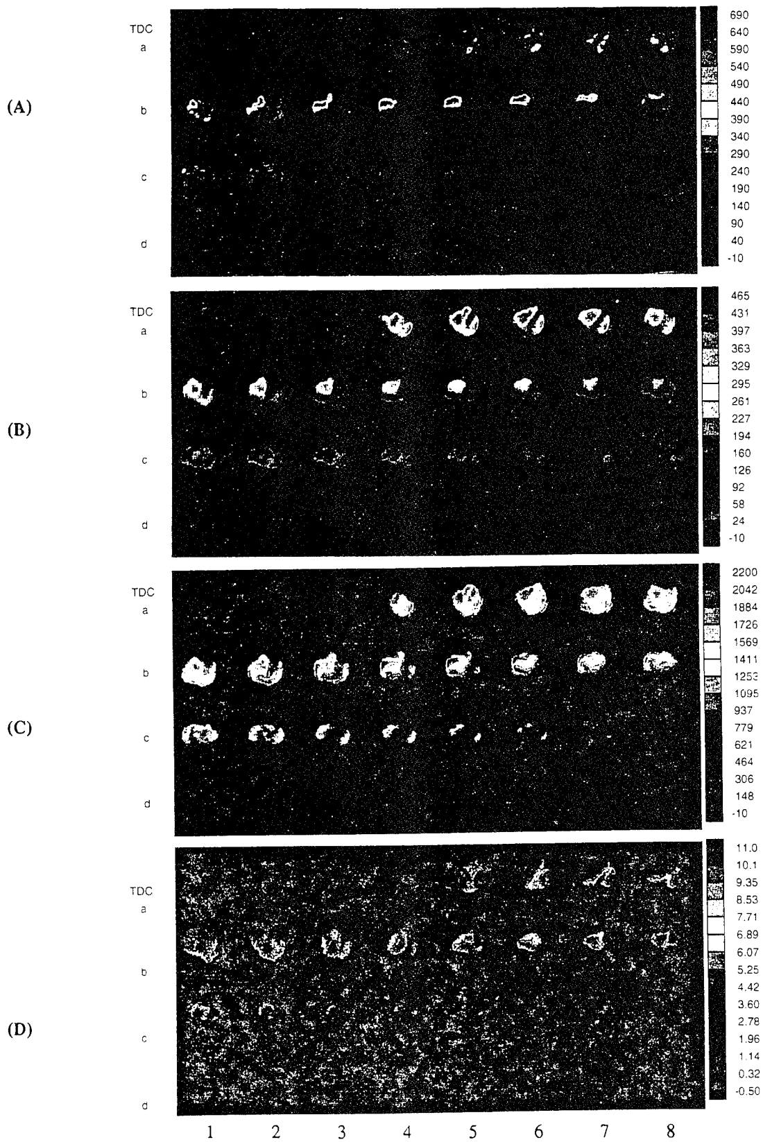
Fig. 6. Instantaneous IR Images Obtained in Exposure Period of 90 \mu sec and Image Interval of 2.5CA from Engine Speed of 500rpm with Injection at 4dTDC. Images Obtained via Bands of (A) 2.2-2.5 \mu m and (B) 4.5-5.5 \mu m. Two-Color Method was Used to Calculate Distributions of (C) Temperature (K) and (D) KL Factor (in a relative scale).
