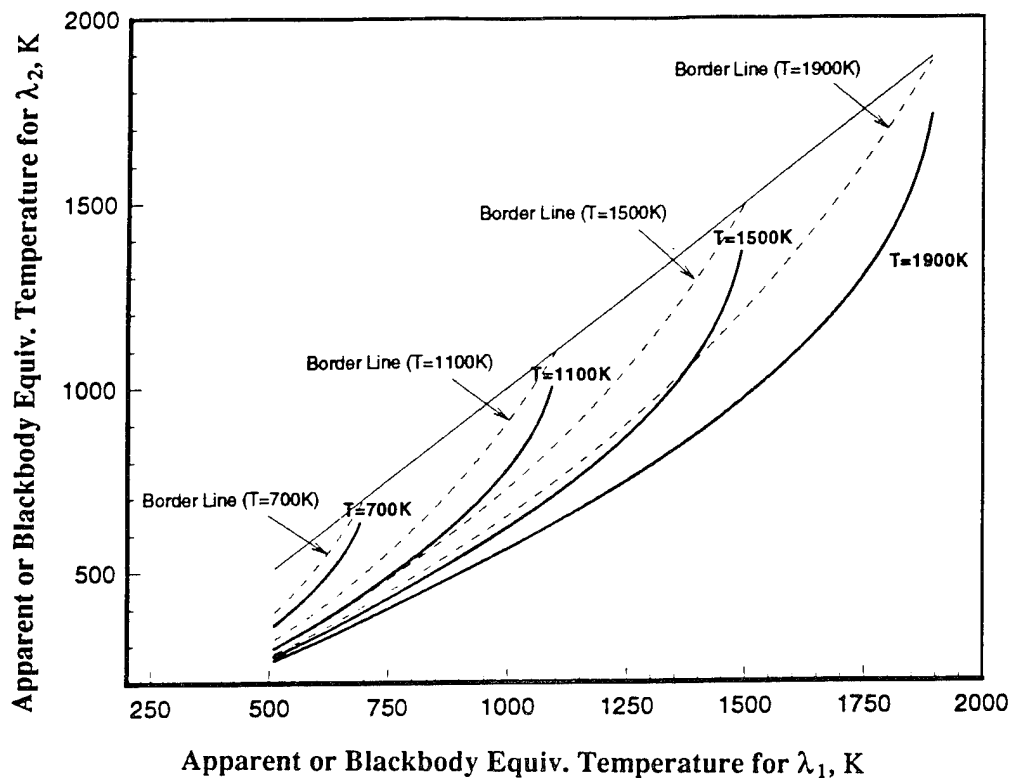
Fig. 4. Solution Domain of Two-Color Method.
