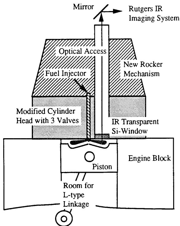
Fig. 2. Schematic Presentation of the Single Cylinder Engine with Optical Access Lined up with the Rutgers High-Speed Imaging System.
