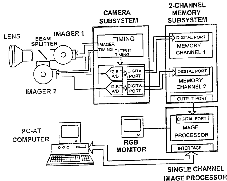
Fig. 2 Dual-band high-speed IR imaging system with memory subsystems.
