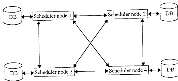
Figure 2: An example of the connections required for a fully connected four-node cooperative peer process network.
