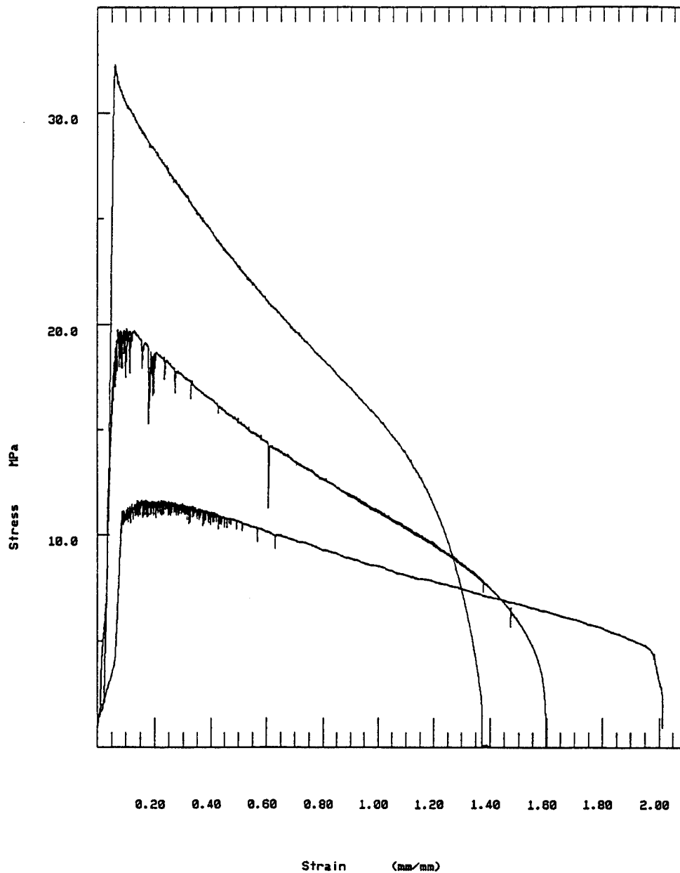
Figure A.1: Stress Versus Strain Curves for Three Tests conducted at 400°C on a material overaged at 450°C for 100 hours. Strain rates of a) 10^{-2} b) 10^{-3} c) 10^{-4} \text{sec}^{-1} .
