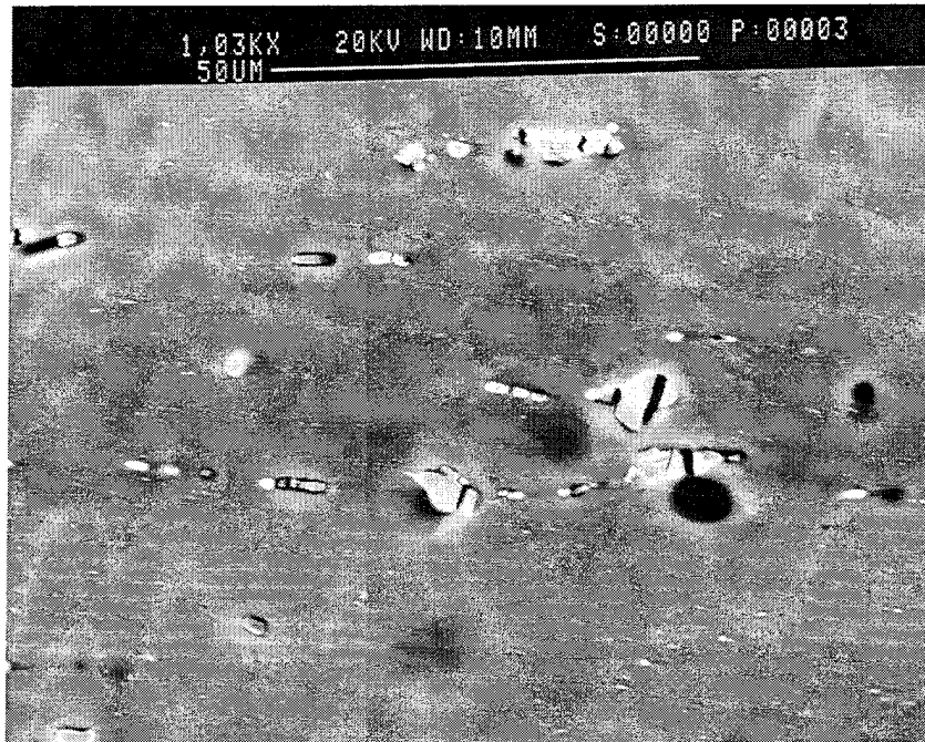
Figure 4.5.b Backscattered electron micrograph of the as received aluminum 2519, showing the \theta precipitates at high magnification.
