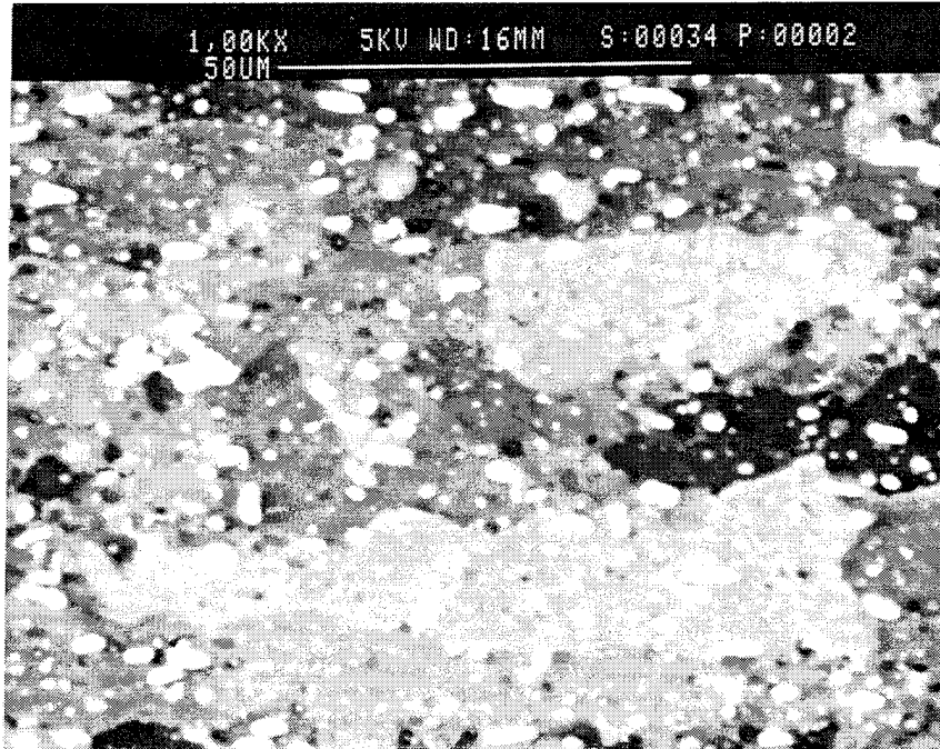
Figure 4.8 Backscattered electron micrograph of a sample overaged at 450°C for 100 hours and then tested at 300°C with a strain rate of 10^{-4} \text{ sec}^{-1} .
