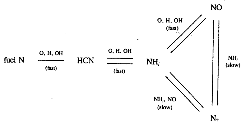
Figure 3-4. Simplified schematic showing (a) HCN as intermediate in conversion of fuel N to NO or \text{N}_2 and, (b) importance of \text{NH}_i to establishing equilibrium gas concentrations.
