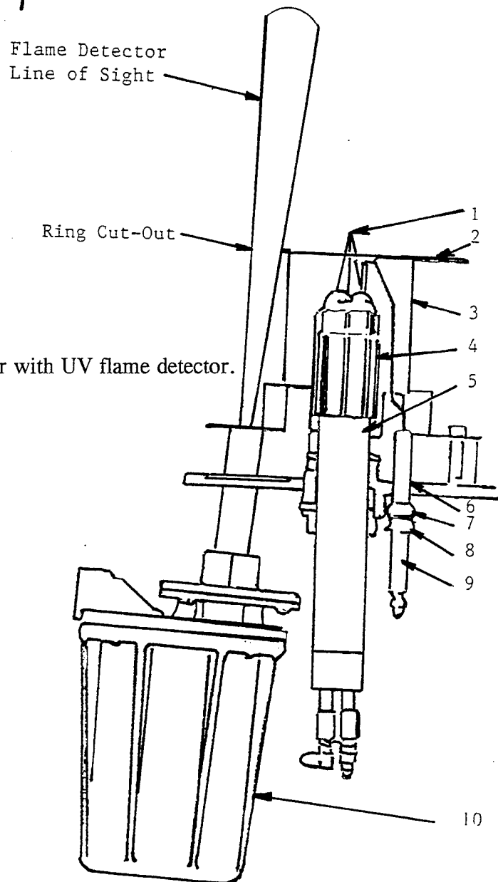
Figure 4-6. Pressure atomization.
