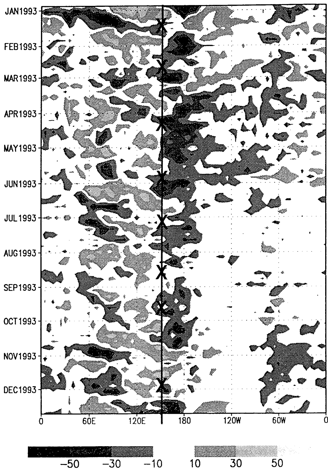
Fig. 19. Time-longitude section ( 5^{\circ}N - 5^{\circ}S ) of anomalous OLR (Adapted from the Climatic Diagnostics Bulletin, December 1993 Issue). Anomalies are computed for each pentad (average of 5 day period) with units of W m^{-2} . The solid black line represents the average longitude of the three DF's while the "X's" correspond to the peaks in the filtered Kavieng total flashes series.
