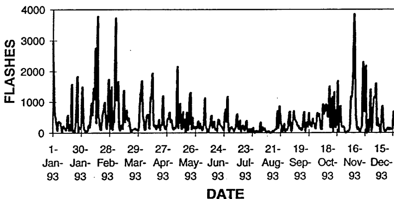
Rabaul Ocean Sector Lightning Time Series (Corrected-1993)
