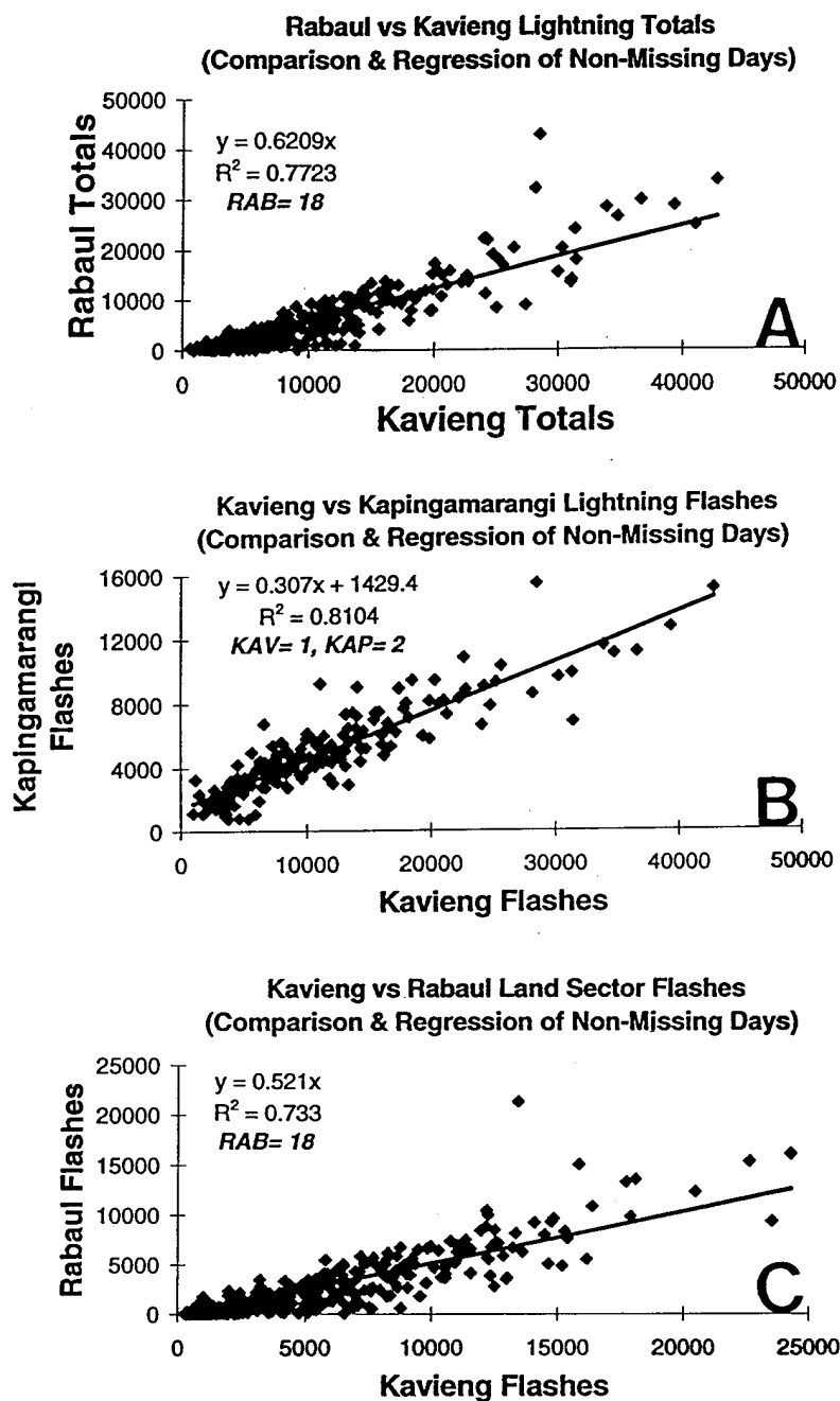
Fig. 10. Six linear regressions using all nine time series; total flashes on total flashes (a&b), land on land flashes (c&d), and ocean on ocean flashes (e&f). RAB = "#", KAV = "#", and KAP = "#" corresponds to how many data gaps each regression was used for.
