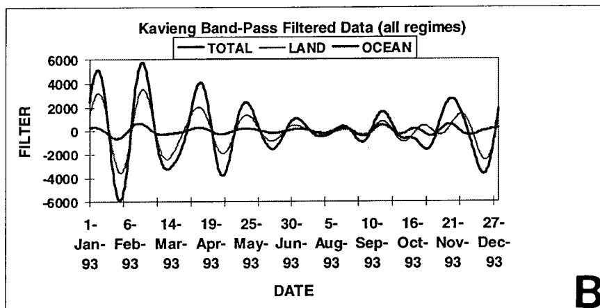
Fig. 18. Filtered Kavieng series superimposed on total flashes (a). Total, land, and ocean filters (b) for Kavieng.
