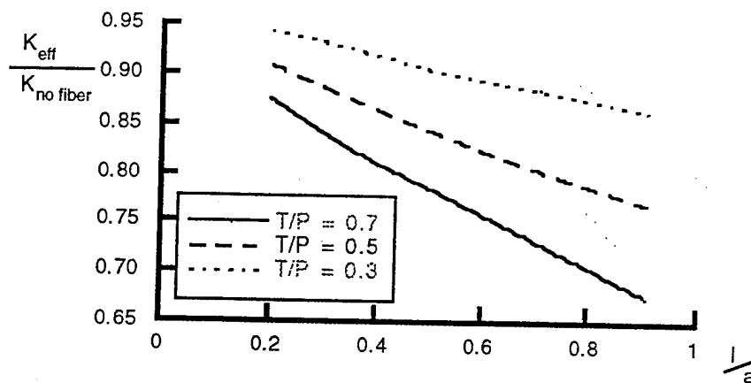
FIGURE 7. COMPUTATIONAL PREDICTION OF THE VARIATION IN NORMALIZED STRESS INTENSITY FACTOR WITH THE FRACTION OF THE CRACK LENGTH BRIDGED BY FIBERS FOR THREE VALUES OF CLOSING TRACTION. ALL THE CURVES REPRESENT 50% VOLUME FRACTION OF FIBERS IN THE NICALON-GLASS COMPOSITE.
