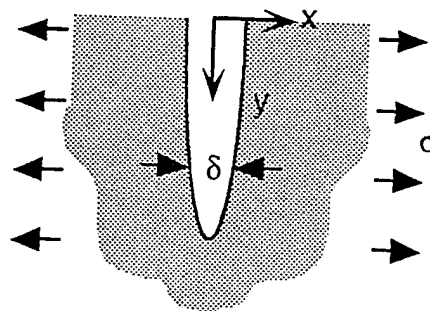
FIGURE 2. AN EDGE CRACK SUBJECT TO MODE I TENSION. THIS GEOMETRY MATCHES THE EXPERIMENTS.
