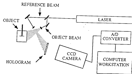
Figure 4. Holographic apparatus and image acquisition system.
