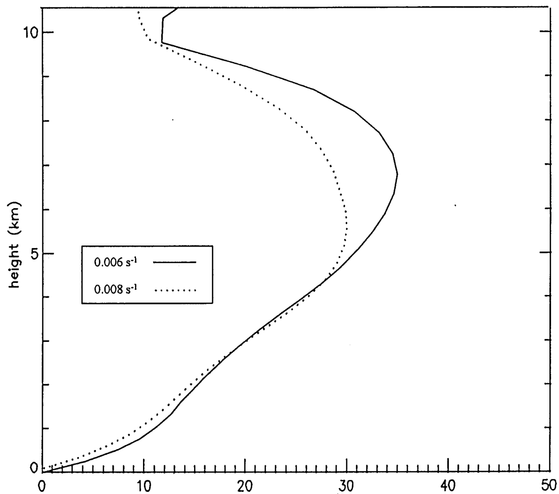
FIG. 14b. Same as FIG. 14a for the 08 km EL, 0.006 s -1 and 0.008 s -1 shear cases.
