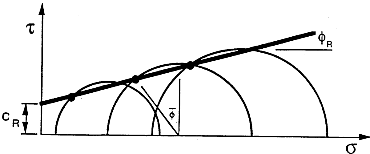
b - R ("Total Stress") Envelope Through Points Representing Stresses on the Failure Plane.
