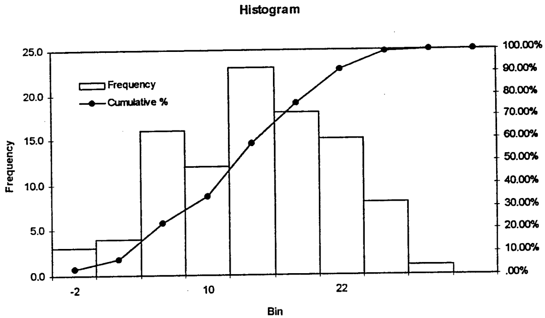
Figure 8: Medium Iceberg Melted Size Histogram
