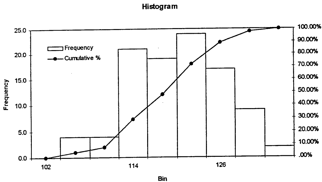
Figure 9: Large Iceberg Melted Size Histogram
