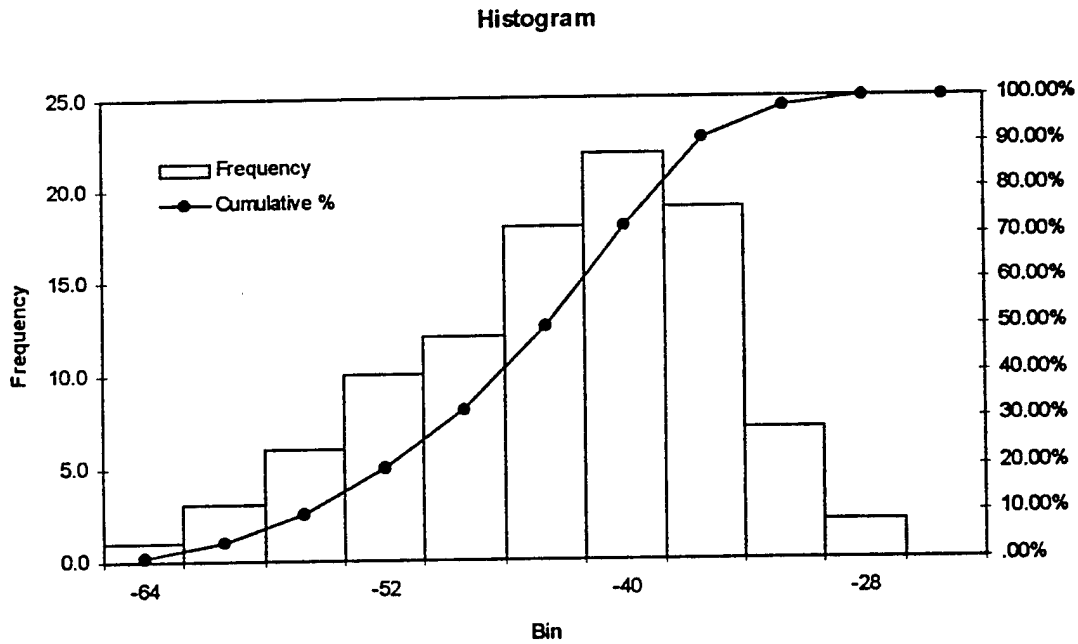
Figure 7: Small Iceberg Melted Size Histogram
