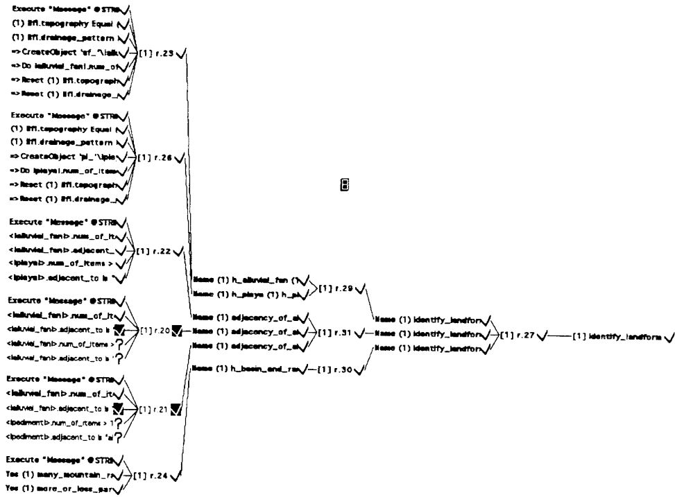
Figure 14. Backward chaining with multiple hypothesis
