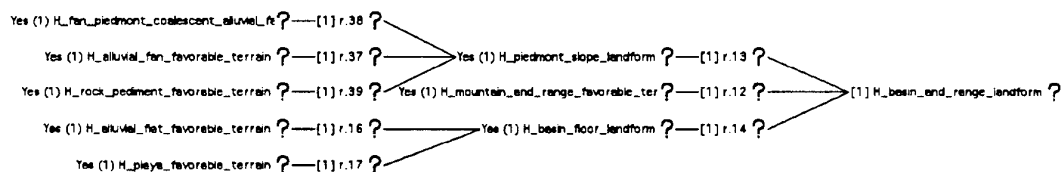
Figure 23. A partial reasoning path connecting the hypothesis of the Basin and Range province and the alluvial fan landform
