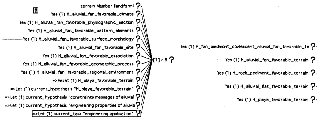
Figure 26. An evidence combining rule for the alluvial fan favorable terrain
