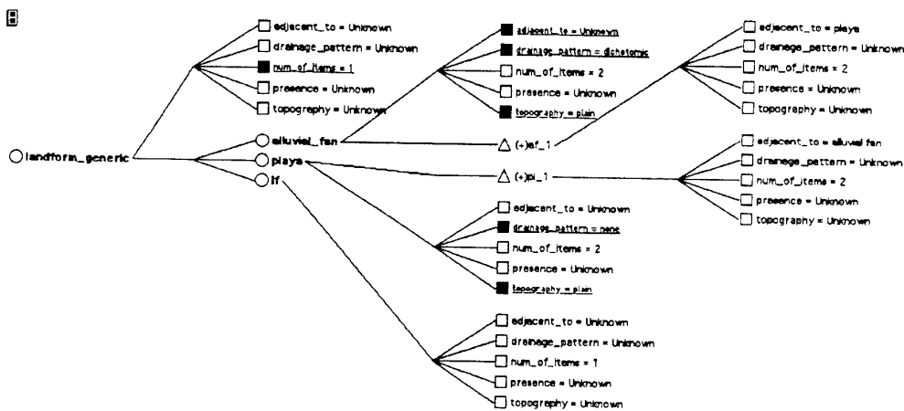
Figure 3. Dynamic objects (af_1, pl_1): instances of two landform classes created during the expert system consultation
