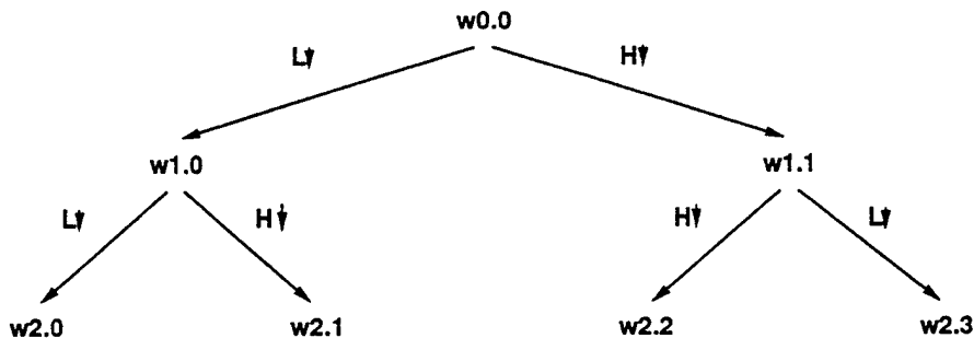
Figure 3: Pyramid algorithm for wavelet packet table.
